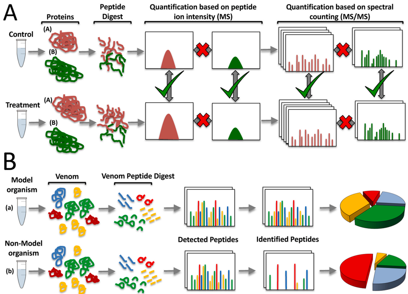
Fig. 5. Panel A , generalised representation of label-free shotgun proteomics. Both control and treatment samples are separately prepared and subjected to individual mass spectrometric analysis. In shotgun, or bottom-up proteomics, proteins are enzymatically digested into peptides, often with trypsin, prior to mass spectrometry. Label-free quantification (LFQ) is based on comparison of the areas of the peptide precursor ions of the same peptide, or by counting the number of fragment ion spectra of the same protein, in the different analyses. Appropriate comparisons are highlighted by the green ✓. Red X highlight that label-free strategies are not appropriate for determining the abundances of different proteins in a single sample: in this example, there is no change in abundance for protein B between control and treatment samples, whereas protein A is most abundant in the treated sample. Panel B , simulation of the different outcomes of label-free quantification of the same shotgun-generated tryptic venom peptidome when a species-specific genomic/transcriptomic reference database is available (a) or not (b) to match the tryptic peptide set.
