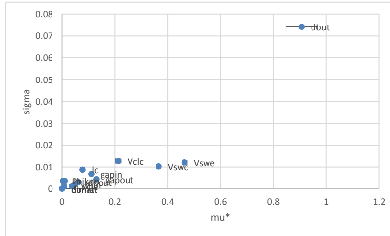
Figure 4. Morris analysis of the computed power variability
