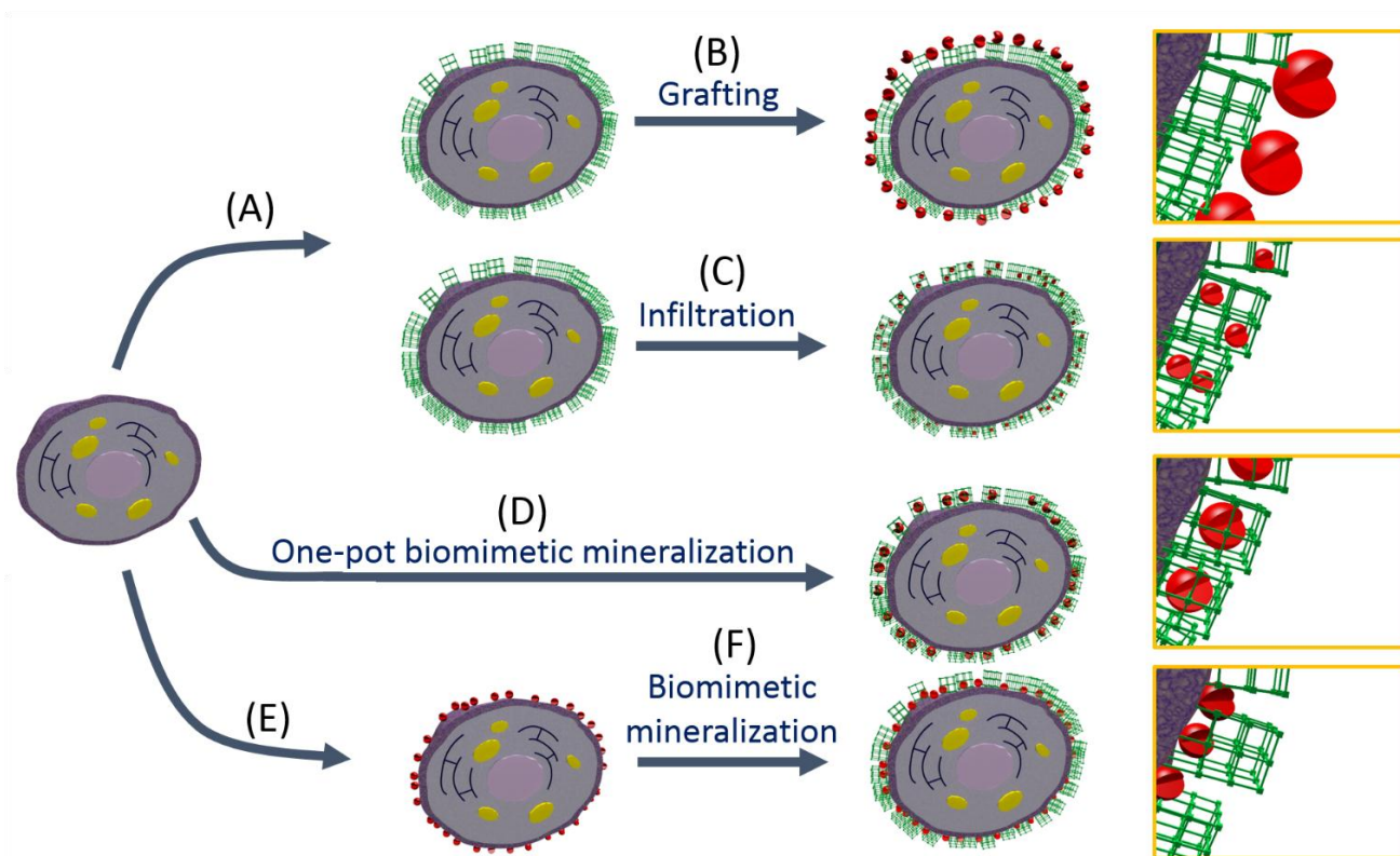
Figure 3. A) A cell can be coated with a metal–organic framework (MOF) via biomimetic mineralization, then B) enzymes can be grafted to the surface of the framework. C) If the framework pore and pore aperture size are large enough, enzymes can be introduced into the MOF via infiltration. D) A biomimetic mineralization procedure in the presence of enzyme results in a shell where the biomacromolecules are encapsulated in a single step. Finally, E) enzymes can be directly immobilized on the surface of the cell, followed by F) biomimetic mineralization to afford a cell/enzyme system.
