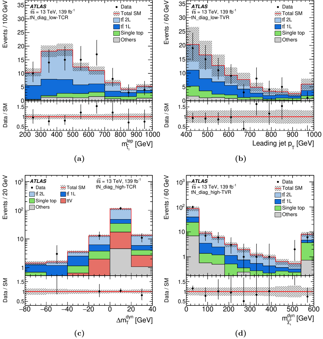
Figure 6. Selected kinematic distributions in tN\_diag\_low and tN\_diag\_high TCRs and TVRs: (a) m_{l_1}^{lep} in the tN\_diag\_low TCR, (b) leading jet p_T in the tN\_diag\_low TVR, (c) \Delta m_T^{dyn} in the tN\_diag\_high TCR, (d) m_{\chi_1^0}^{dyn} in the tN\_diag\_high TVR. The distributions shown are post-fit, i.e. each background is scaled by a normalisation factor obtained from a background-only likelihood fit to the CRs (see table 14). The hatched area around the total SM prediction and the hatched band in the Data/SM ratio include all statistical and systematic uncertainties. The last (first) bin contains overflows (underflows).
