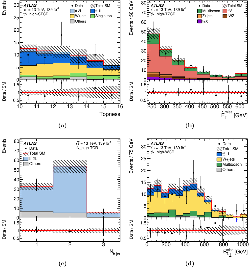
Figure 4. Selected kinematic distributions in tN_{\text{high}} CRs: (a) topness in the STCR, (b) \tilde{E}_T^{\text{miss}} in the TZCR, (c) N_{b\text{-jet}} in the TCR, (d) E_{T,\perp}^{\text{miss}} in the WCR. The distributions shown are post-fit, i.e. each background is scaled by a normalisation factor obtained from a background-only likelihood fit to the CRs (see table 14). The hatched area around the total SM prediction and the hatched band in the Data/SM ratio include all statistical and systematic uncertainties. The last (first) bin contains overflows (underflows).
