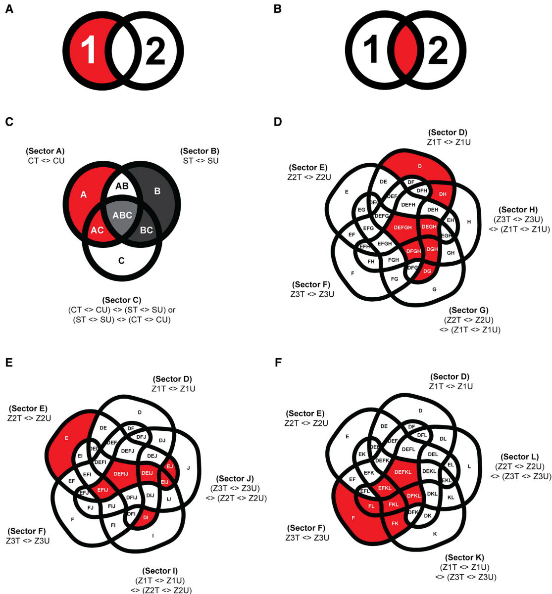
Figure 2. Design of GLM and Subsetting for the DEG or DAM Determination.
