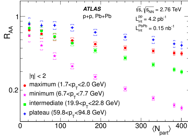
Figure 16. The R_{AA} values plotted as a function of \langle N_{\text{part}} \rangle measured in four transverse momentum intervals corresponding to the maximum R_{AA} ( 1.7 < p_T < 2.0 GeV), minimum R_{AA} ( 6.7 < p_T < 7.7 GeV), intermediate R_{AA} ( 19.9 < p_T < 22.8 GeV) and plateau of R_{AA} ( 59.8 < p_T < 94.8 GeV). The statistical uncertainties, which are smaller than the size of markers in all but a few cases, are shown with vertical bars and the systematic uncertainties with brackets.
