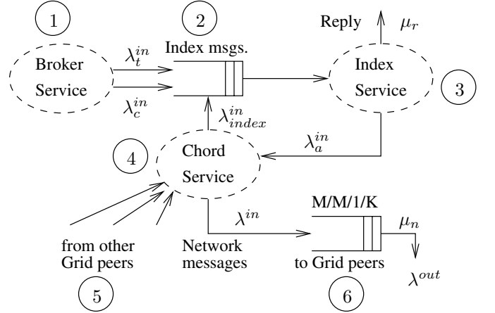
Fig. 6. Network message queueing model at a Grid peer i .
