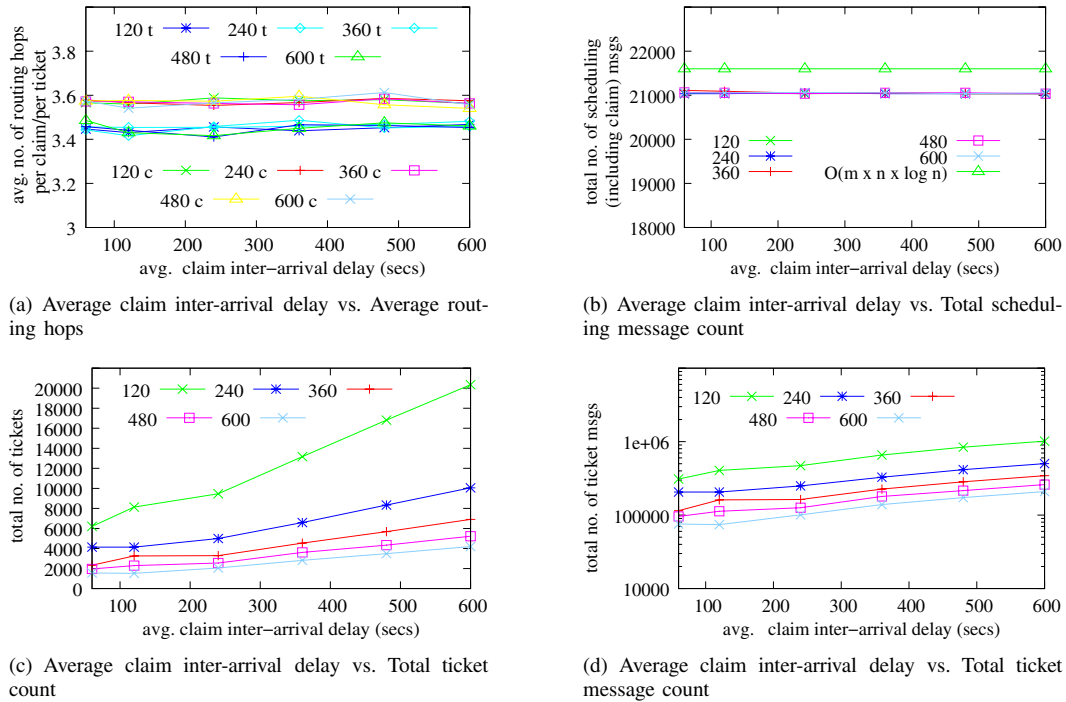
Fig. 8. Effect of \frac{1}{\lambda_c^{in}} and \frac{1}{\lambda_t^{in}} on different performance metrics (Network perspective).
