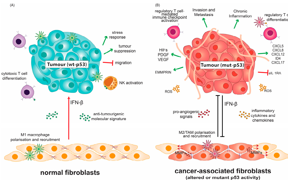
Figure 2. Mutant p53 alters its immunogenic niche. The tumour microenvironment is comprised of cellular and molecular components which shape the immune niche of the growing tumour. (A) Normal fibroblasts help mediate immunosurveillance by modulating anti-tumour immune cell infiltration and employing the IFN- \beta /p53 axis of regulation to activate anti-tumour responses. (B) Mutant p53 in the tumour alters the crosstalk between the tumour and its microenvironment, suppressing IFN- \beta signalling and supporting pro-angiogenic signalling. This altered crosstalk converts normal fibroblasts into tumour-supporting cancer-associated fibroblasts with altered p53 functionality. The altered transcriptional program of cancer-associated fibroblasts (CAFs) supports pro-tumorigenic signalling and extracellular matrix remodelling. The demographic and functionality of infiltrating immune cells is consequently shifted to favour immunosuppression, ultimately leading to a chronically inflamed environment and enhanced migration and invasion.
