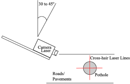
Fig. 2. Cross-hair laser pattern to detect pothole and uneven surfaces.
