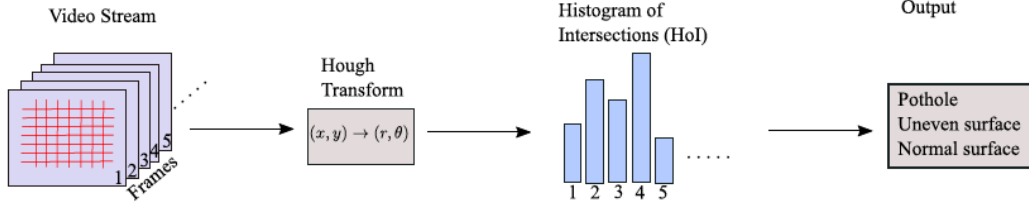
Fig. 1. Overview of the proposed approach to detect potholes and uneven surfaces.
