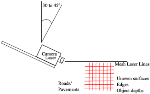
Fig. 3. Mesh laser pattern to detect pothole and uneven surfaces.
