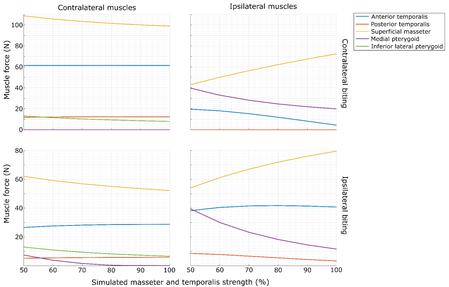
Figure A.D.5: Resultant muscle forces for the anterior temporalis, posterior temporalis, superficial masseter, medial pterygoid and inferior lateral pterygoid muscles when the maximum isometric force of the temporalis and masseter sub-regions are modelled as 50%, 60%, 70%, 80%, 90% and 100% of their full capacity.
