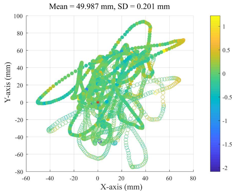
Figure A.B.1: DMD precision, evaluated from differences between calculated and actual sensor spacing as two sensors glued to a plate were moved through the magnetic field capture volume.
