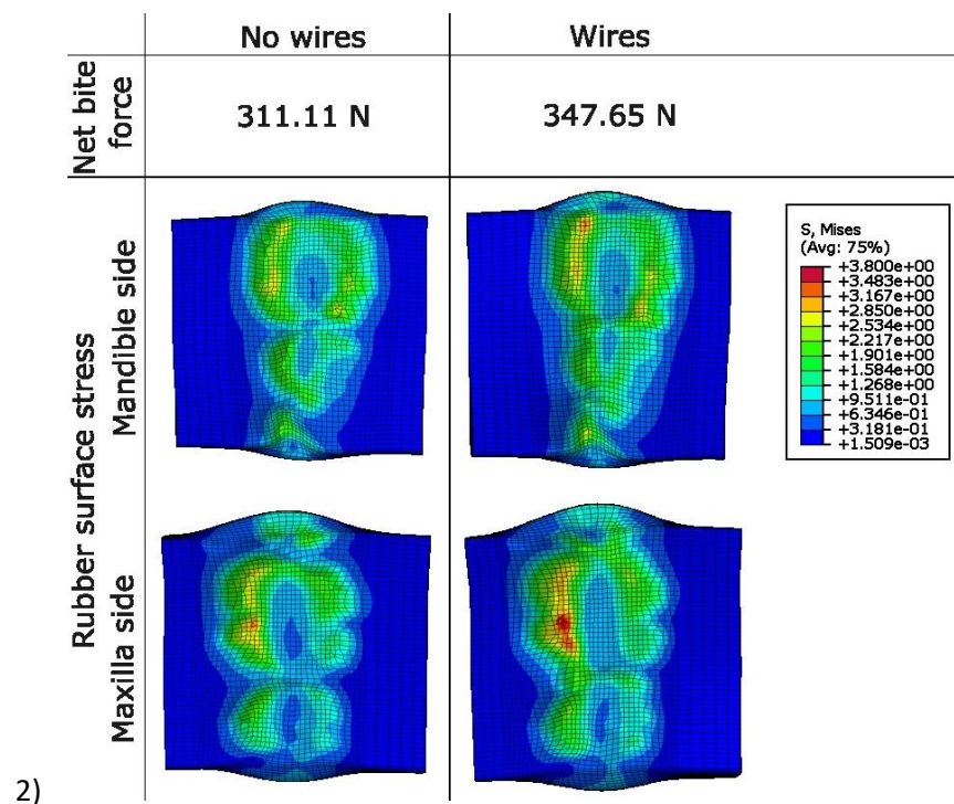
Figure A.D.4: Results of sensitivity analysis studying the effects of the mouthpiece wires on bite force results.
