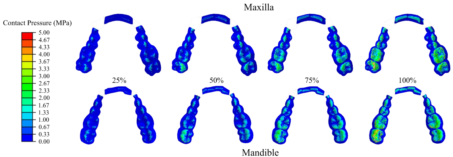
Figure 4.6: Evolution of the contact pressure distribution along the maxillary (top row) and mandibular (bottom row) dental arches at 25%, 50%, 75% and 100% of the mean chewing cycle. Contact pressure values are given in MPa.
