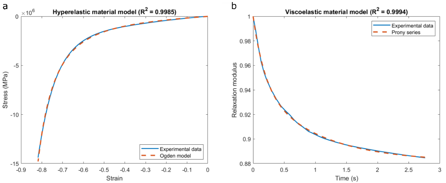
Figure A.D.1: Material model fit to experimental data. (a) Hyperelastic material response, Ogden model ( N=1 ) fit to average experimentally measured stress-strain data. (b) Viscoelastic material response, Prony series ( N=2 ) fit to average experimentally measured stress-relaxation data.
