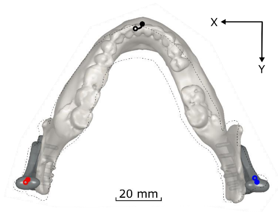
Figure A.C.2: Example of maximum lateral excursion towards the right projected onto the transverse plane for a bilateral total TMJ replacement patient. Dashed line represents mandible position at maximum occlusion position, rendered mandible represents mandible position at maximum lateral excursion position. Open circles represent landmarks at the mouth closed position, closed circles represent landmarks at the maximum lateral position. Black, red, and blue lines indicate incisal, left condyle and right condyle trajectories respectively.
