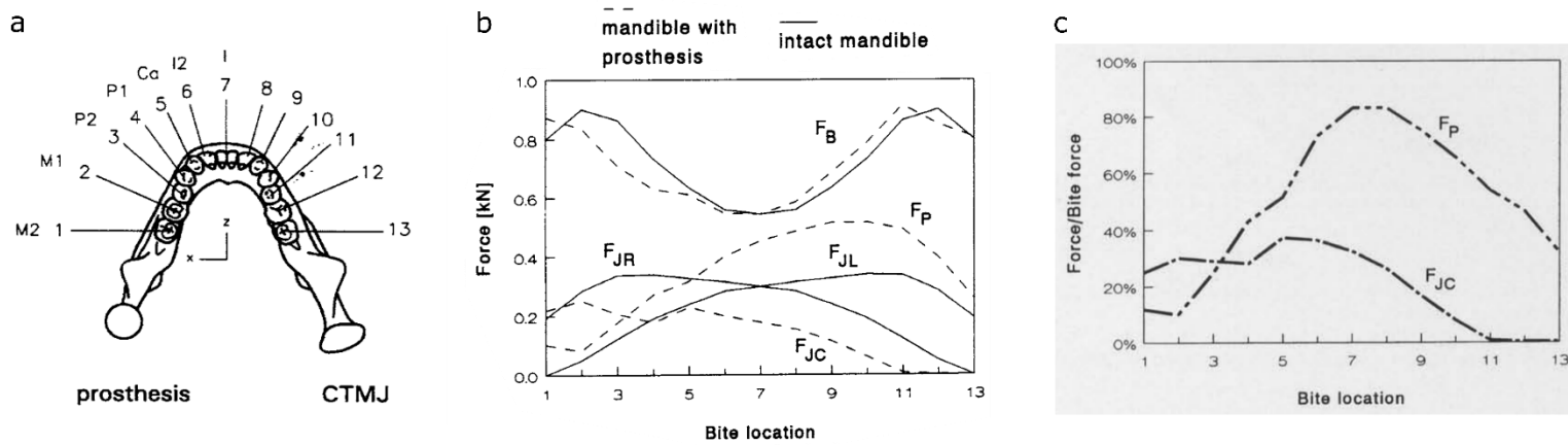
Figure 2.13: Cranial view of mandible showing bite locations numbered 1 to 13 (a). Maximum bite force and corresponding TMJ reaction force as a function of bite location for an intact mandible and for a unilateral TMJ prosthesis (b). Prosthetic and contralateral joint reaction forces normalised against the maximum bite force, as a function of bite location (c). Where F_B = maximum bite force, F_{JL} and F_{JR} = left and right TMJ reaction force for an intact mandible, F_P and F_{JC} = prosthetic and contralateral joint reaction force of a unilateral TMJR patient, M = molar, P = premolar, C = canine, I = incisor. Figure adapted from Van Loon et al. (1998).
