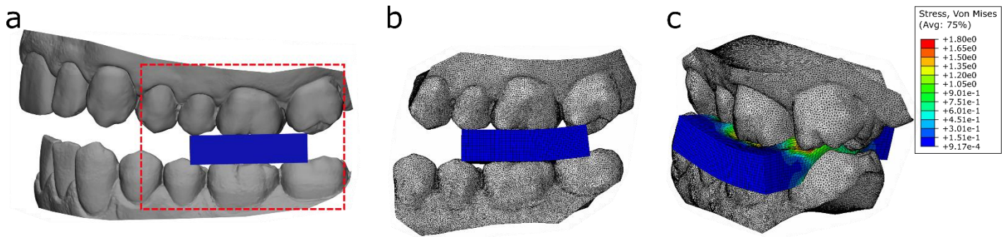
Figure 6.2: Three-dimensional model of the participants mandibular and maxillary teeth with rubber held between the first molars (a), finite element model of the first molars (grey) and rubber (blue) constructed from the laser scan data (b), and the finite element model of the first molars compressing the rubber sample in a maximum force bite (c). The finite element model includes only the teeth that will contact the rubber for computational efficiency, indicated by the red dashed lines.
