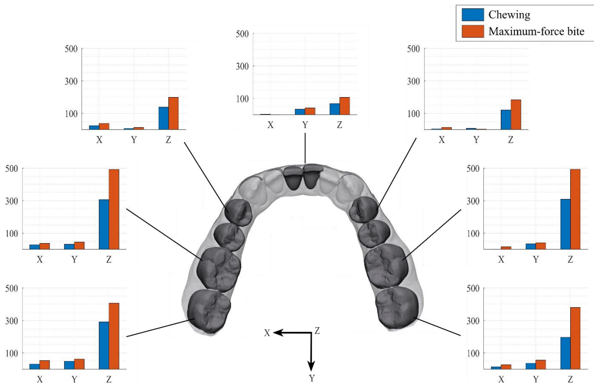
Figure 4.5: Tooth-specific mandibular bite forces for mean chewing and maximum-force bite tests. Data are given for the incisors, premolars, first molars and second molars. All forces are given in Newtons; X, Y and Z represent the lateral (left), posterior and superior directions, respectively.
