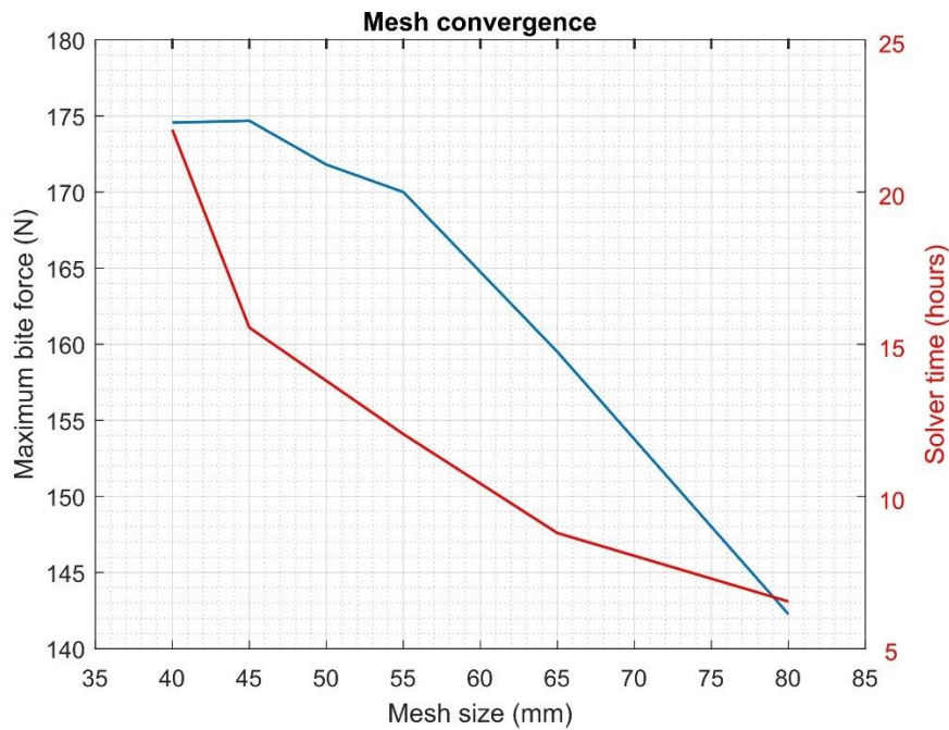
FigureA.D.2: Mesh convergence analysis results showing the maximum bite force (blue) and solver time (red) variation with mesh size.
