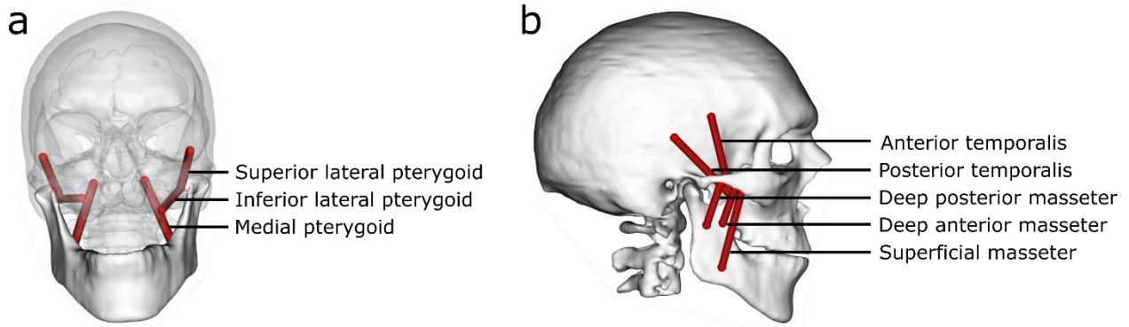
Figure 6.3: Rigid-body musculoskeletal model illustrating the pterygoid sub-regions in the frontal plane (a) and temporalis and masseter sub-regions in the sagittal plane of healthy controls (b). The superior and inferior sub-regions of the operated lateral pterygoid muscles are removed in the models of unilateral total TMJR patients.
