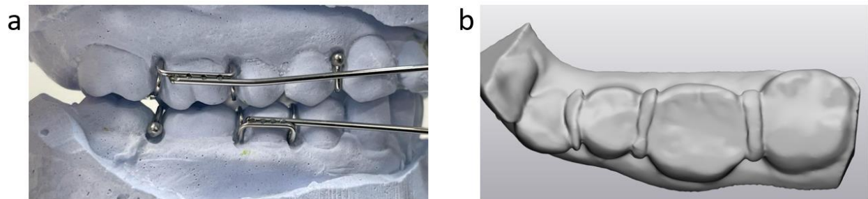
Figure A.D.3: Dental stone casts with mouthpieces attached showing maximum occlusion position (a), model of mandibular teeth with 0.7 mm wires between the teeth (b).
