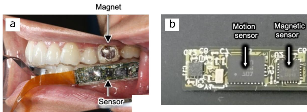
Figure 3.7: Intraoral photograph of the electromagnetic tracking device developed by Morikawa et al (2022) (a). Photograph of the sensor module, attached to the mandibular teeth, including a magnetic and motion sensor (b). Images adapted from Morikawa et al. (2022).
