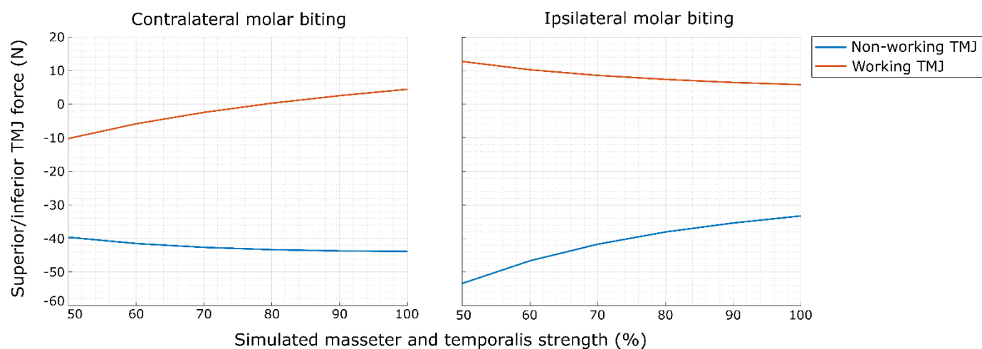
Figure A.D.6: TMJ loading when the maximum isometric force of the temporalis and masseter sub-regions are modelled as 50%, 60%, 70%, 80%, 90% and 100% of their full capacity.
