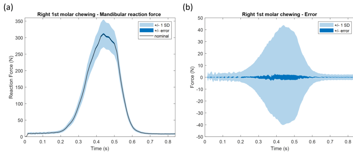
Figure A.B.2: (a) Effect of propagated kinematic measurement errors on the calculated bite force of the right 1st molar across the chewing cycle. (b) Resulting mean error in bite force calculation (dark blue) and error from \pm 1 SD of the kinematic measurement error (light blue).
