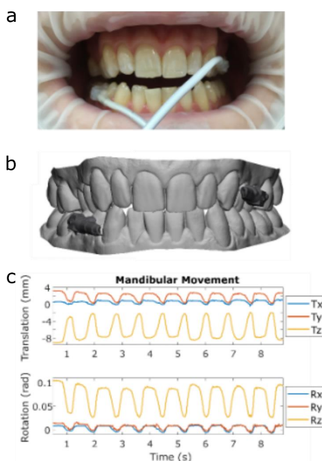
Figure 3.4: Magnetic DMD system with magnetic sensors fixed to participant's premolars using dental cement (a). The motion of these sensors can be registered to subject-specific dental geometry reconstructed from an intra-oral scanner (b), resulting in three orthogonal translations and rotations of the mandible with respect to the maxilla during habitual mastication (c). Data given are expressed about an anatomic coordinate system with the x-direction, y-direction and z-direction aligned with the lateral, anterior and superior directions, respectively.
