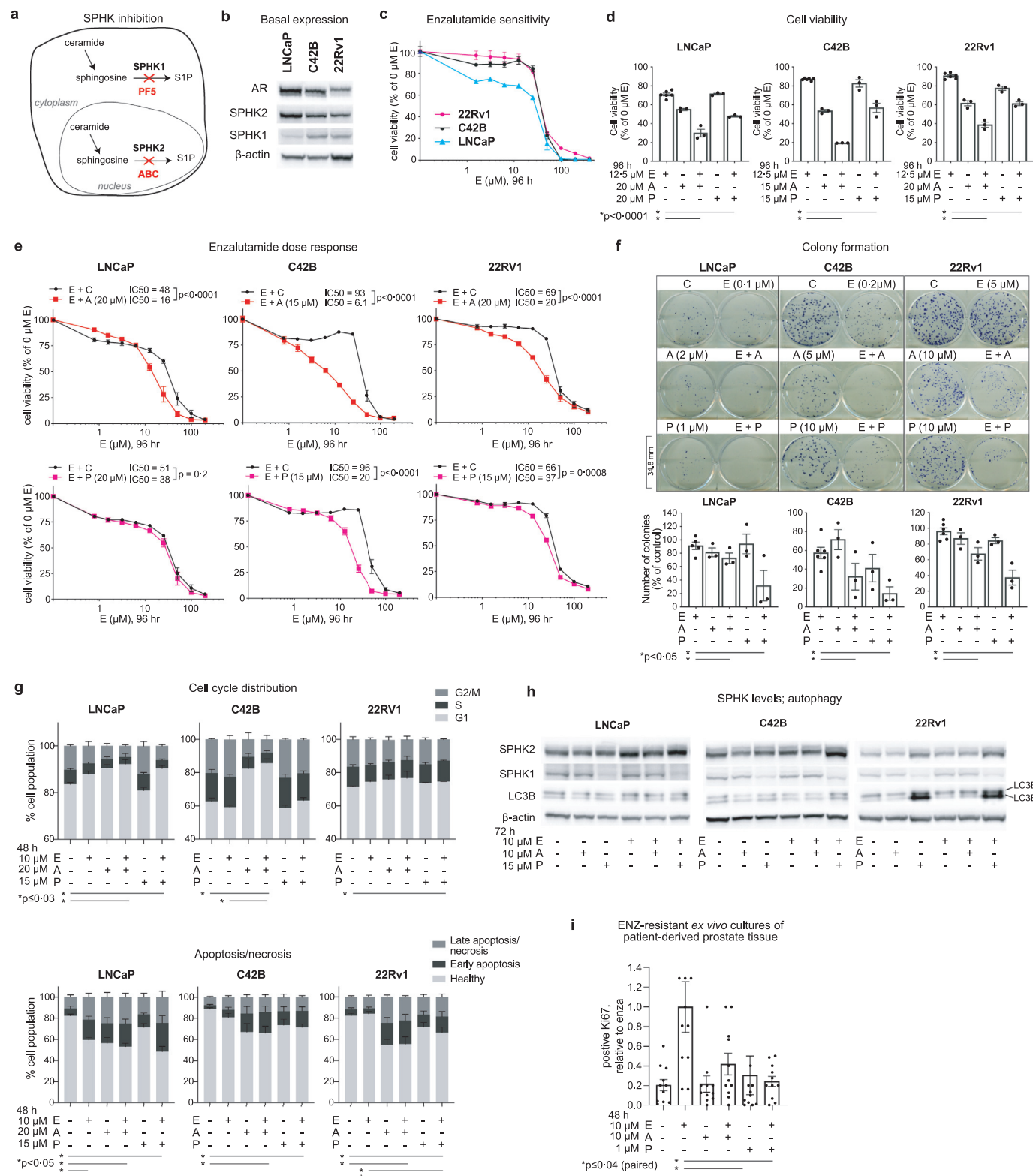
Fig. 3. ENZ-SPHK inhibition reduces viability of prostate cancer cells (figure abbreviations: C, vehicle control; E, ENZ; P, PF5; A, ABC): (a) sphingosine kinase (SPHK) inhibition – PF5 inhibits SPHK1 which is present in the cytoplasm, whereas ABC inhibits SPHK2 which is predominantly present in the nucleus, thus blocking the conversion of sphingosine into S1P; (b) representative Western blot confirming the expression of AR, SPHK1 and SPHK2 (original whole blot displayed in Supplementary S4); (c) ENZ dose-response curves demonstrating differences in sensitivity of the cell lines; (d) cell viability after 96 h treatment of SPHK inhibitors \pm ENZ, * t -test p < 0.0001 ; (e) ENZ dose-response curves of combination treatment; (f) representative photos of colony formation, and number of colonies formed after treatment with SPHK inhibitors \pm ENZ, *one-tail t -test p < 0.05 ; (g) distribution of cell cycle phases and percentage of apoptotic/necrotic cells after 48 h treatment with SPHK inhibitors \pm ENZ, * t -test p \leq 0.05 for at least one of the subsets; (h) representative Western blots of SPHK1, SPHK2 and LC3B (original whole blots displayed in Supplementary S4); (i) percentage of Ki67 in explants cultured from fresh primary prostate tumours of 11 patients (mean \pm standard error), *paired t -test p \leq 0.04 . Dose response curves and bar graphs are mean \pm standard error of 3–4 replicates unless shown otherwise. P -values are calculated by two-tail t -test, unless stated otherwise.
