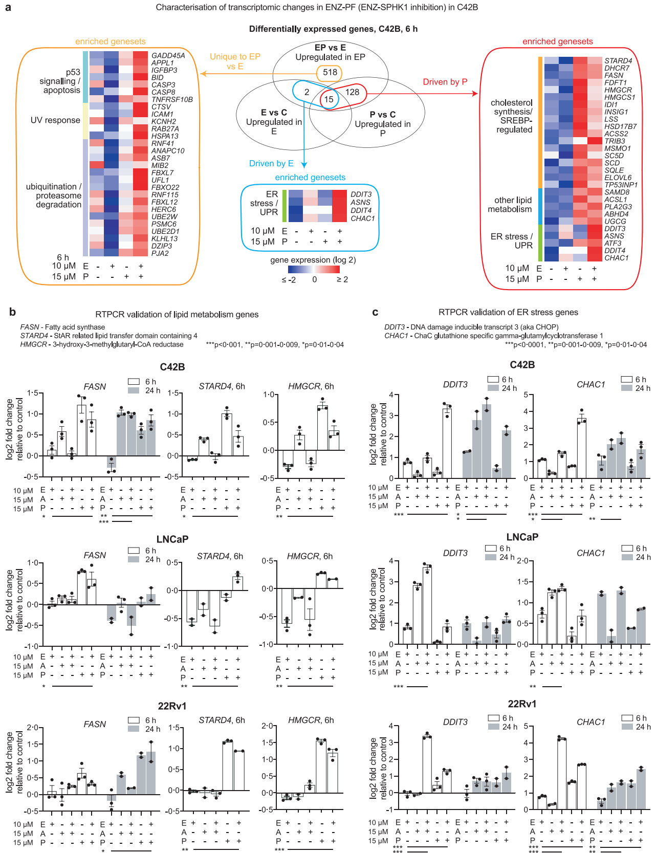
Fig. 4. Transcriptomic changes induced by ENZ-SPHK inhibition in cell lines (figure abbreviations: C, vehicle control; E, ENZ; P, PF5; A, ABC): (a) Venn diagram of upregulated genes in C42B treated with ENZ, PF5 or control for 6 h, and heatmap of the expression of enriched genes from the Venn diagram partitions; (b) & (c) RTPCR quantitation of representative genes associated with lipid metabolism and ER stress in C42B, 22Rv1 and LNCaP cells after 6 or 24 h treatment. P -values are from two-tail t -tests. Bar graphs are mean \pm standard error.
