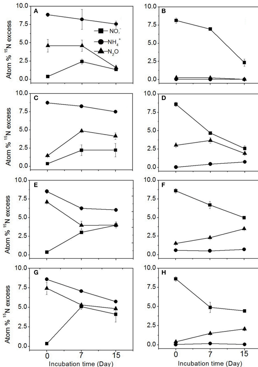
FIGURE 2 | 15 N enrichment of \text{N}_2\text{O} , \text{NH}_4^+ , and \text{NO}_3^- in the 15 N labeled \text{NH}_4^+ and \text{NO}_3^- treatments during the incubation. (A,C,E,G) represent the 15 N-labeled \text{NH}_4^+ treatment in the sugarcane, vegetable, dairy pasture, and cereal cropping soils, respectively. (B,D,F,H) represent the 15 N labeled \text{NO}_3^- treatment in the sugarcane, vegetable, dairy pasture, and cereal cropping soils, respectively. Error bars represent standard error.
