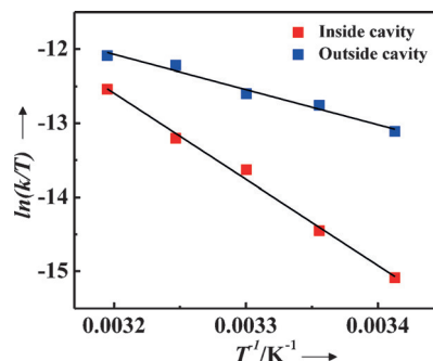
Figure 4. The reaction rate ([PTA] = 2.53 M, \hbar\Omega_{\text{VR}} = 98 cm −1 ) as a function of temperature (Eyring equation plot) for reactions inside the ON resonance cavity (red squares) and outside the cavity (blue squares).
