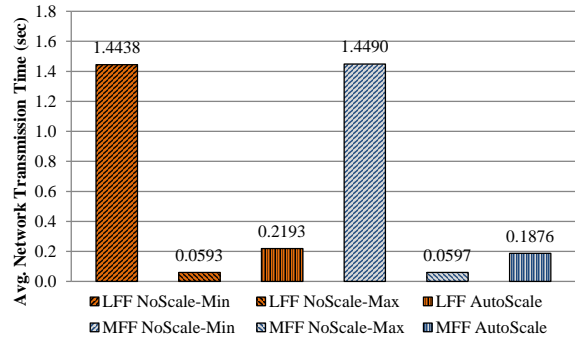
(d) Average Network delays through SFC policies without IDS
