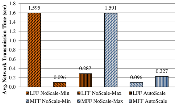
(c) Average Network delays enforcing through SFC policies.
