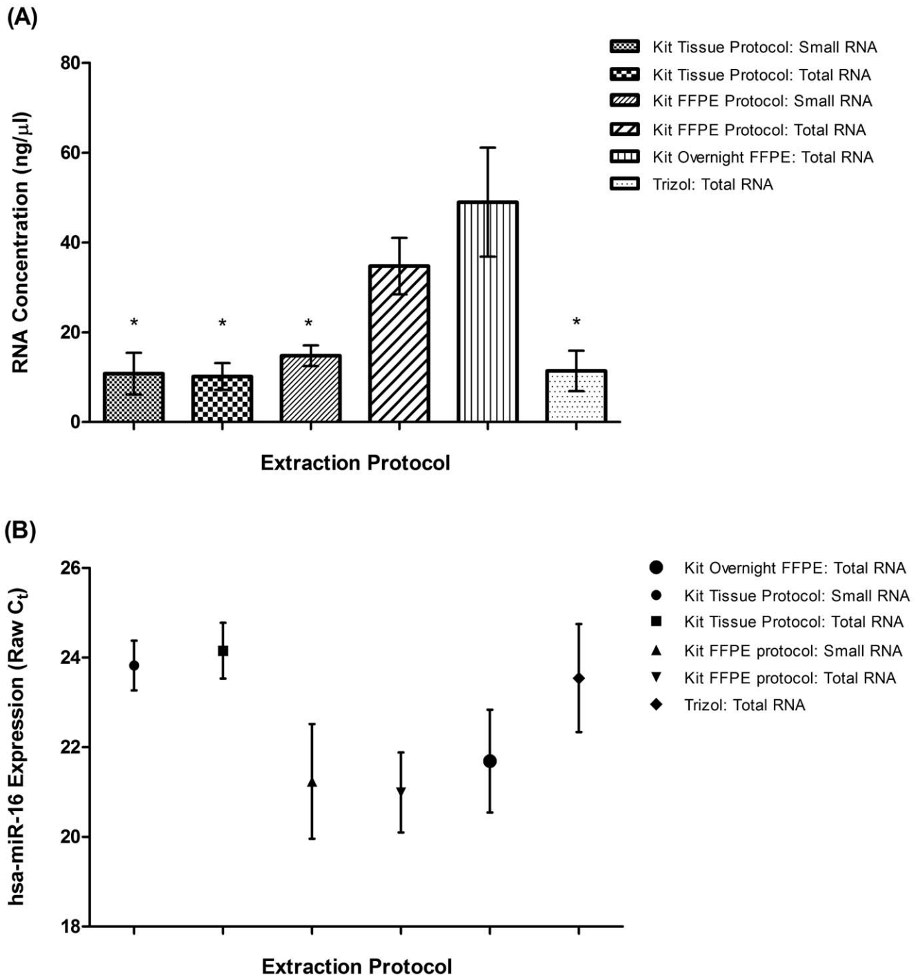
Figure 2. A comparison of RNA extraction methods for the evaluation of RNA concentration (ng/μl) and miRNA expression from archived bone marrow aspirate slides. The comparison of miRNA extraction methods from matched unstained archived bone marrow smears ( n = 6 or n = 8 patients; Table S3). Six different methods were used based on traditional TRIzol or using the Roche High Pure miRNA Column extraction kit (Table 1). (A) Comparison of Total RNA yield from experimental extraction protocols. The average RNA concentration was measured by NanoDrop (ng/μl \pm s.e.m.). Kit Total RNA extraction methods with a Proteinase K digestion ('FFPE protocol') are higher in RNA yield compared to kit methods without a digestion step ('Tissue protocol'), or when extracting small RNA only. These methods are also significantly better than TRIzol extractions. The archived slide extraction method with the highest RNA yield was the Roche kit 'isolation from FFPE Tissue' Total RNA extraction with an overnight Proteinase K digestion. * Indicates RNA concentration is significantly different to the Kit Overnight FFPE: Total RNA protocol. (B) Comparison of hsa-miR-16 expression from experimental extraction protocols. The average expression of our reference gene (hsa-miR-16) measured by qRT-PCR (raw C_t \pm s.e.m.). Raw C_t value tracks with total RNA yield, whereby as the concentration of RNA increases the C_t value decreases. This analysis shows extractions with a Proteinase K digestion return a lower C_t value compared to extractions without a digestion step. TRIzol extractions also return a higher C_t value than the Proteinase K digestion protocols. doi:10.1371/journal.pone.0042951.g002
