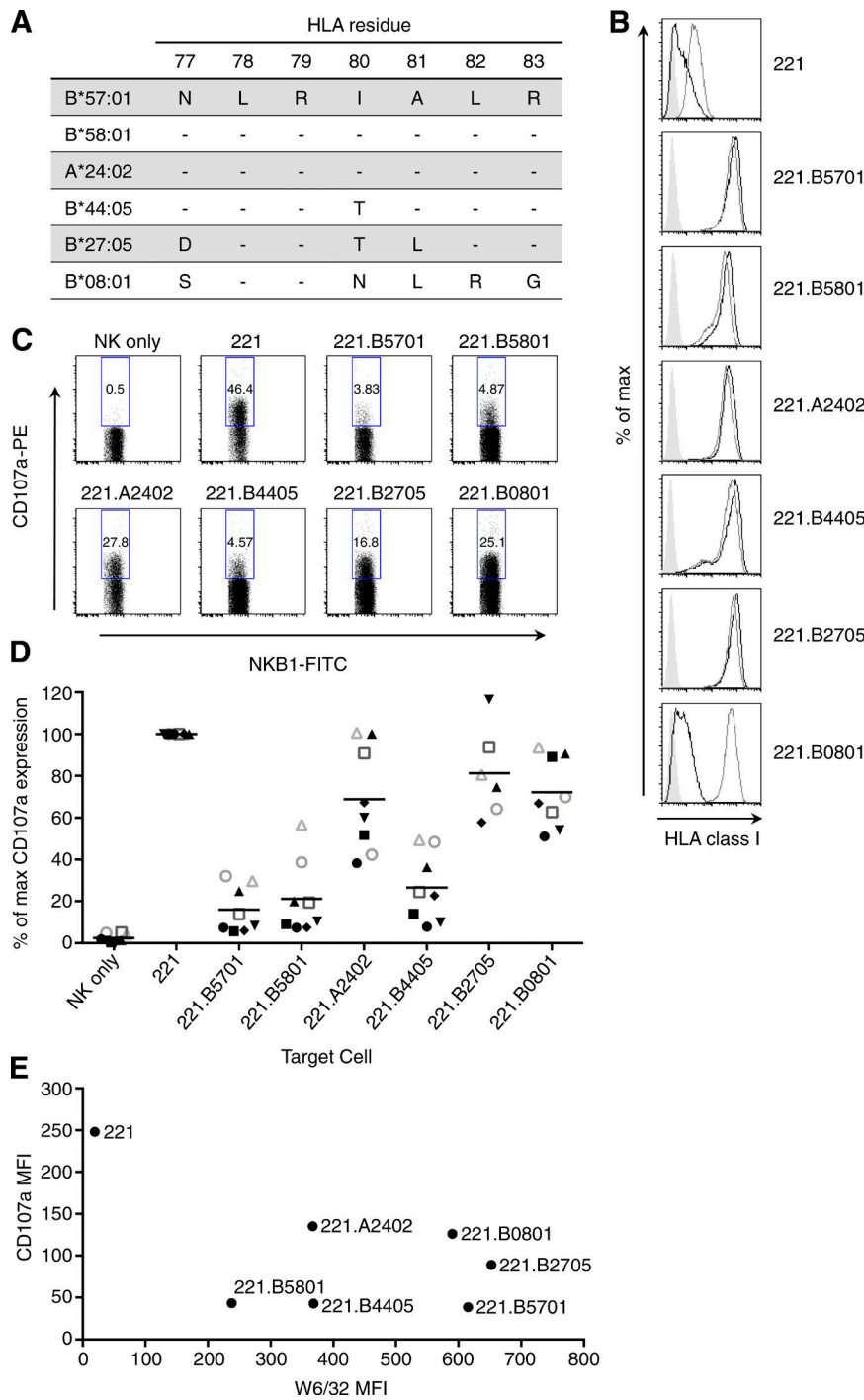
Figure 1. Inhibition of KIR3DL1 + NK cells varies with HLA-Bw4 expressing targets. (A) Amino acid sequences across residues 77–83 of transfected HLA-I molecules. (B) The surface expression of transfected HLA-I molecules was confirmed by staining with W6/32 (gray histograms) or anti-Bw4 (black histograms) mAbs followed by anti-mouse IgG-FITC. Filled gray histograms represent background staining with secondary antibody alone. (C and D) KIR3DL1 + NK cells were sorted from eight donors and expanded with IL-2. Equal numbers of KIR3DL1 + NK cells and 221 transfected target cells were cultured with the addition of anti-CD107a for 4 h in the presence of monensin. CD107a expression was then examined by flow cytometry, gating on CD56 + /NKB1 + cells. (C) Representative flow cytometric plots showing CD107a expression. Values indicate the percentage of cells expressing CD107a. (D) Normalized CD107a expression after co-culture of KIR3DL1 + NK cells with transfected or parental 221 cells where the response to untransfected 221 cells was adjusted to 100%. Horizontal lines indicate mean. Data are pooled from six independent experiments. (E) The MFI of W6/32 versus the MFI of subsequent CD107a expression is plotted for each 221 transfectant for a representative donor.
