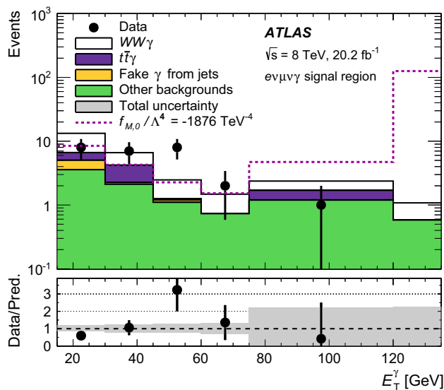
Fig. 3 Observed and expected transverse energy distribution of the photon with the highest E_T in the ev\mu\nu\gamma signal region. The data are shown together with the predicted signal and backgrounds. Also indicated is the expected event yield for a reference model describing aQGCs with f_{M,0}/\Lambda^4 = -1876 \text{ TeV}^{-4} (see Sect. 8). The last bin contains all overflow events. The lower panel shows the ratio of the observed number of events to the sum of expected signal and background events as well as the corresponding uncertainties
