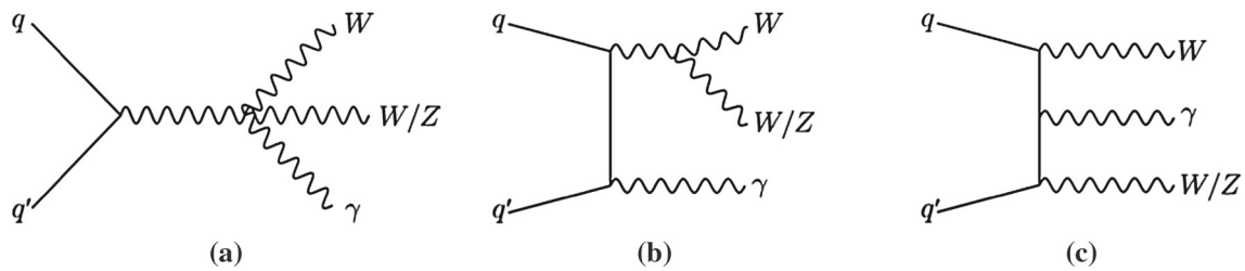
Fig. 1 Examples of Feynman diagrams of WV\gamma production at the LHC. In a the quartic vertex is shown, while b , c depict the production from radiative processes
