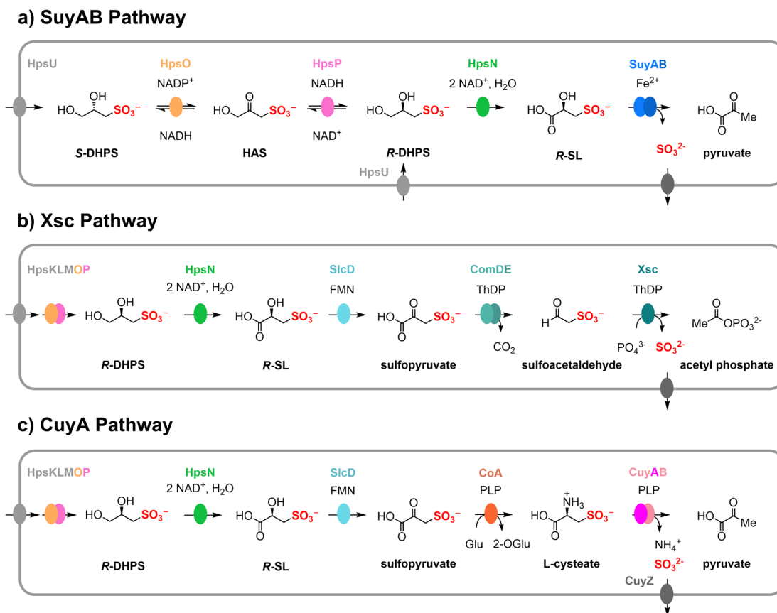
Fig. 2 Various DHPS biomineralization pathways via SL as an intermediate, formed through the action of DHPS-3-dehydrogenase (HpsN). (a) \text{Fe}^{2+} -dependent SL lyase (SuyAB) pathway. (b) Thiamine diphosphate-dependent sulfoacetaldehyde acetyltransferase (Xsc) pathway. (c) PLP-dependent cysteate lyase (CuyA) pathway.
