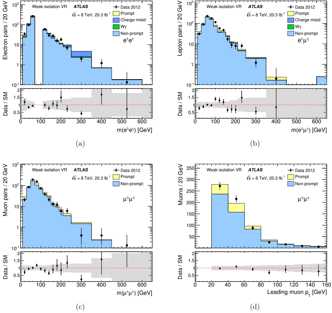
Figure 1. Invariant mass distributions in one of the validation regions (VR) used in the (a) e^\pm e^\pm (b) e^\pm\mu^\pm and (c) \mu^\pm\mu^\pm channels. The p_T distribution for the leading muon in the \mu^\pm\mu^\pm channel is shown in (d). In (a), (c) and (d) the leading lepton of the pair passes the signal isolation cuts while the subleading lepton passes the “weak” isolation cuts (weak isolation on subleading lepton VR). The mass range between 70 GeV and 110 GeV is not included in the e^\pm e^\pm channel as this region is used to estimate the background from charge misidentification. The electron passes the isolation cuts defined for the signal region while the muon passes the “weak” isolation cuts in (b) (weak isolation on muon VR). The data are compared to the background expectations and the lower panels show the ratio of data to the background prediction. The error bars on the data points show the statistical uncertainty and the dashed band shows the total uncertainties of the predictions. The last bin in the histograms includes overflows, and is normalised as though it is 50 GeV wide in (a)–(c) and 20 GeV wide in (d).
