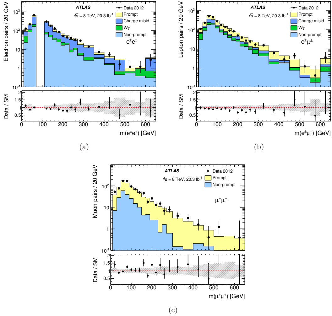
Figure 2. Invariant mass distribution of (a) e^{\pm}e^{\pm} (b) e^{\pm}\mu^{\pm} and (c) \mu^{\pm}\mu^{\pm} pairs as a function of a threshold on the dilepton mass in the same-sign signal region. The mass range between 70 GeV and 110 GeV is not included in the e^{\pm}e^{\pm} channel as this region is used to estimate the background from charge misidentification. The data are compared to the SM expectations and the lower panels show the ratio of data to the background prediction. The error bars on the data points show the statistical uncertainty and the dashed band shows the total uncertainties of the predictions. The last bin in the histograms includes overflows, and is normalised as though it is 50 GeV wide.
