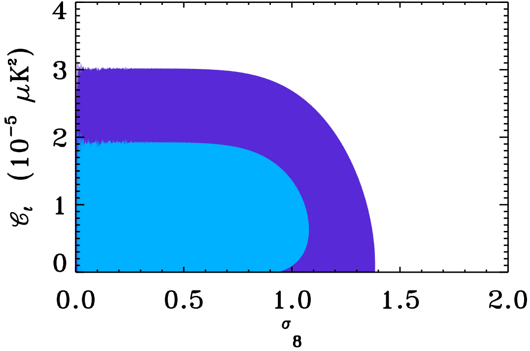
FIG. 3.— The 1\text{-}\sigma and 2\text{-}\sigma contours on the 2D likelihood surface for \sigma_8 and the point source amplitude for the Cluster+Sources mask applied to the APEX-SZ map. The contours include the effects of non-Gaussianity in the SZE. A flat prior on \sigma_8 has been assumed.
