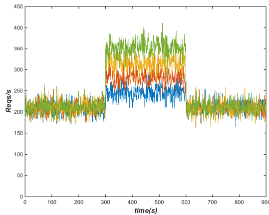
Figure 7. The workloads with flash crowds range from 117% to 183% of the normal load
