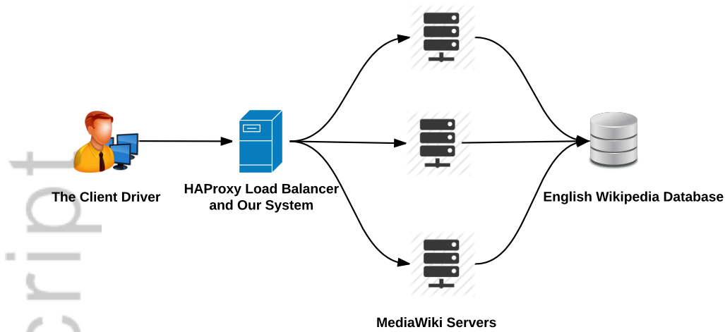
Figure 4. The architecture of the benchmark application
