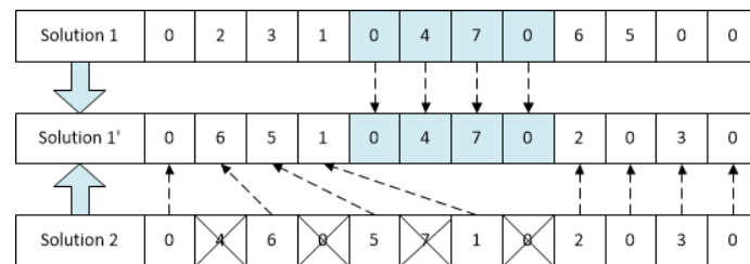
Fig. 4. Crossover operator
