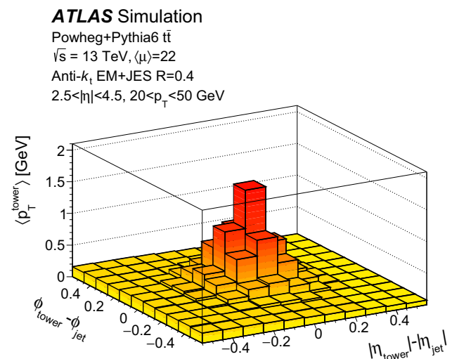
Fig. 7 Distribution of the average tower p_T for hard-scatter jets as a function of the angular distance from the jet axis in \eta and \phi in simulated t\bar{t} events
