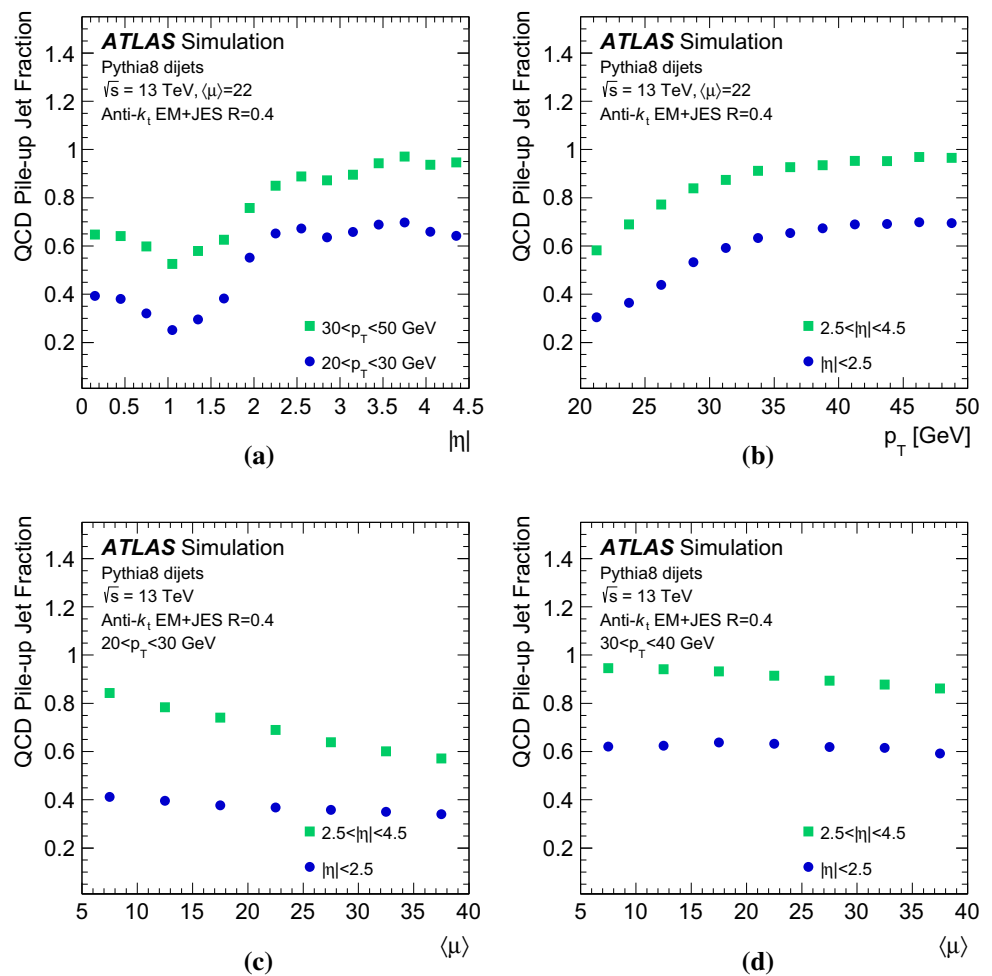
Fig. 4 Fraction of reconstructed pile-up jets classified as QCD pile-up jets, as a function of a |\eta| , b p_T , and c \langle\mu\rangle for jets with 20\text{ GeV} < p_T < 30\text{ GeV} and d 30\text{ GeV} < p_T < 40\text{ GeV} , as estimated in dijet events with PYTHIA8.186 pile-up simulation
