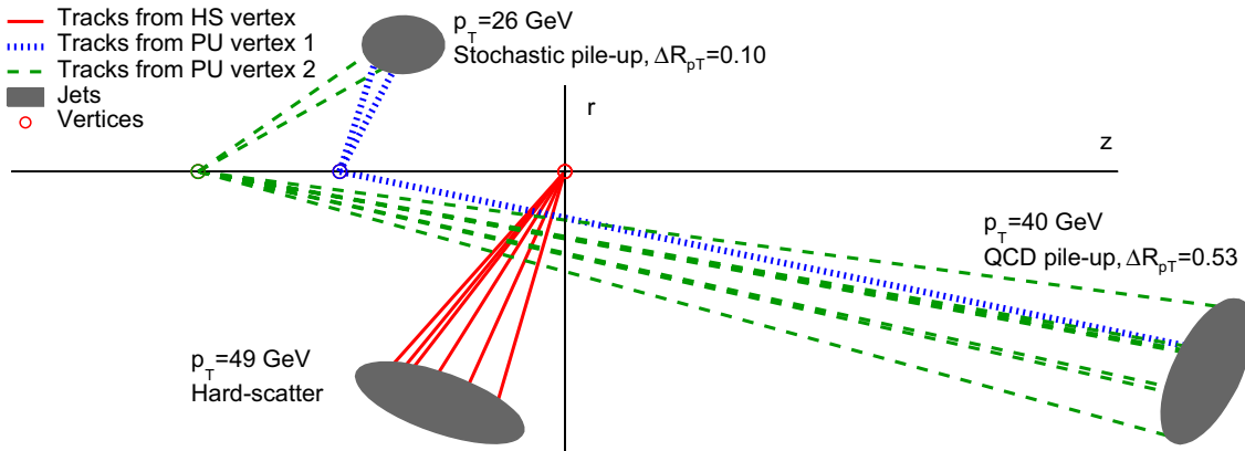
Fig. 2 Display of a simulated event in r - z view containing a hard-scatter jet, a QCD pile-up jet, and a stochastic pile-up jet. The \Delta R_{pT} values (defined in Sect. 5.1) are quoted for the two pile-up jets
