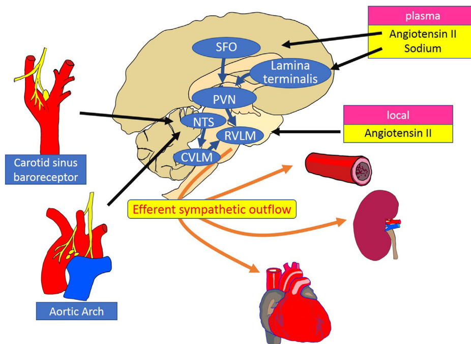
FIGURE 2 | Schematic diagram of the central and peripheral mechanisms of sympathetic regulation of the heart, vessels, and kidneys. The RVLM plays a key role as a cardiovascular centre that receives and integrates peripheral signals providing information on blood pressure, fluid volume, and oxygen saturation. Instant changes in blood pressure are perceived by baroreceptors and transferred to the NTS as an input signal of baroreflex control of sympathetic outflow. Stimulation of the SFO by circulating angiotensin II increases the efferent sympathetic activity through the activation of the PVN and the RVLM neurons. Inhibitory pathways are activated between the lamina terminalis and PVN in response to plasma sodium. Increased activity of the RVLM neurons is transmitted to the intermediolateral cell column of the spinal cord, where peripheral sympathetic nerves to the heart, arteries and kidneys are activated. RVLM, rostral ventrolateral medulla; NTS, nucleus tractus solitarius; CVLM, caudal ventrolateral medulla; PVN, paraventricular nucleus; SFO, subfornical organ.
