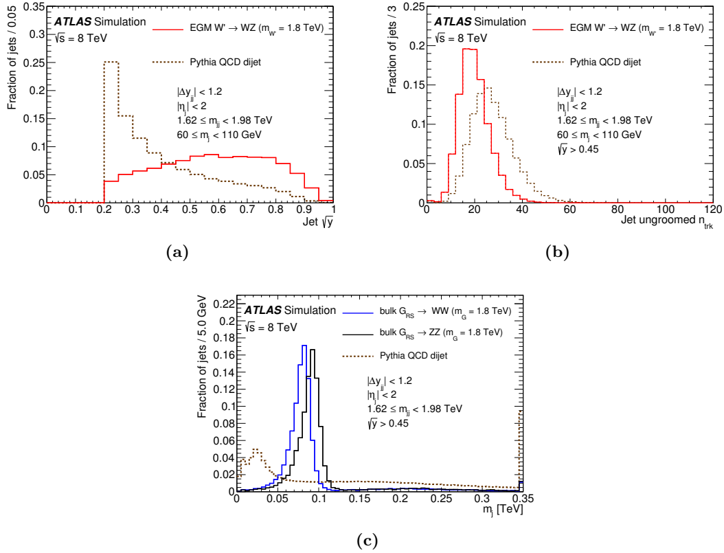
Figure 1. The distribution of the boson-tagging variables (a) subject momentum balance \sqrt{y} , (b) number of tracks n_{\text{trk}} matched to the jet, and (c) mass m_j of the groomed jet, in simulated signal and background events. The signal and background distributions are normalised to unit area, and the last bin of each histogram includes the fraction of events falling outside of the displayed range. Requirements are placed on the events used to ensure that the kinematics of the signal and background events are comparable.
