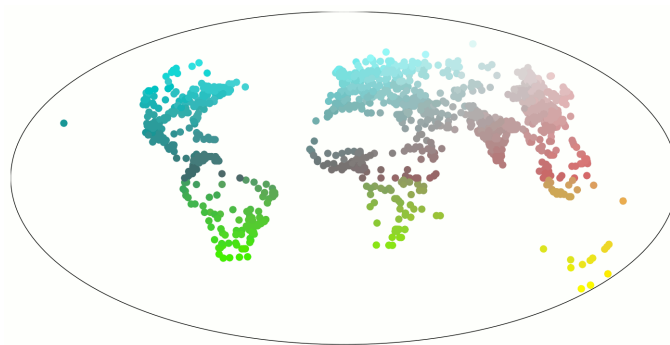
Figure 2. Latitude–longitude–based colour scheme for plotting neural network predictions of cities similar to Melbourne and Sydney.
