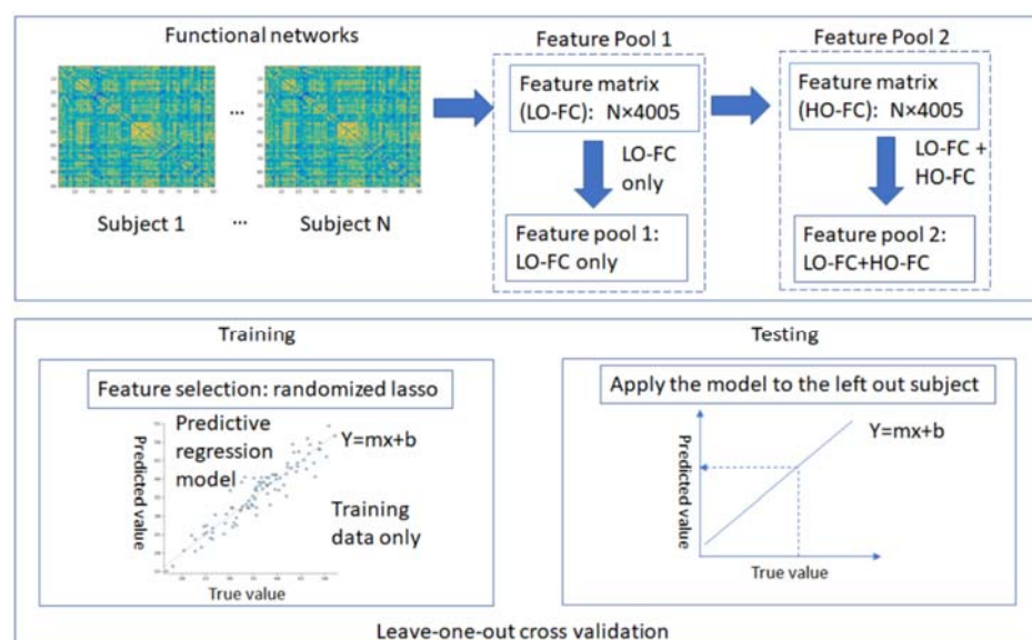
Figure 1. Flow chart of the framework.
