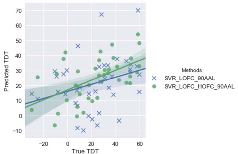
Figure 2. Plots of predicted vs. true Tactile Discrimination Test (TDT) scores by employing support vector regression (SVR) with either LOFC or LOFC + HOFC with feature pools (cerebellum excluded). Correlation coefficients, r , between predicted and true TDT scores are 0.54 and 0.31 for SVR_LOFC_HOFC_90AAL, SVR_LOFC_90AAL, respectively. Note: SVR_LOFC_HOFC_90AAL represents the SVR model using both LOFC and HOFC features based on automated anatomical labelling (AAL) atlas, while SVR_LOFC_90AAL represents the SVR model using LOFC features only based on AAL atlas. LOFC = low-order functional connectivity. HOFC = high-order functional connectivity.
