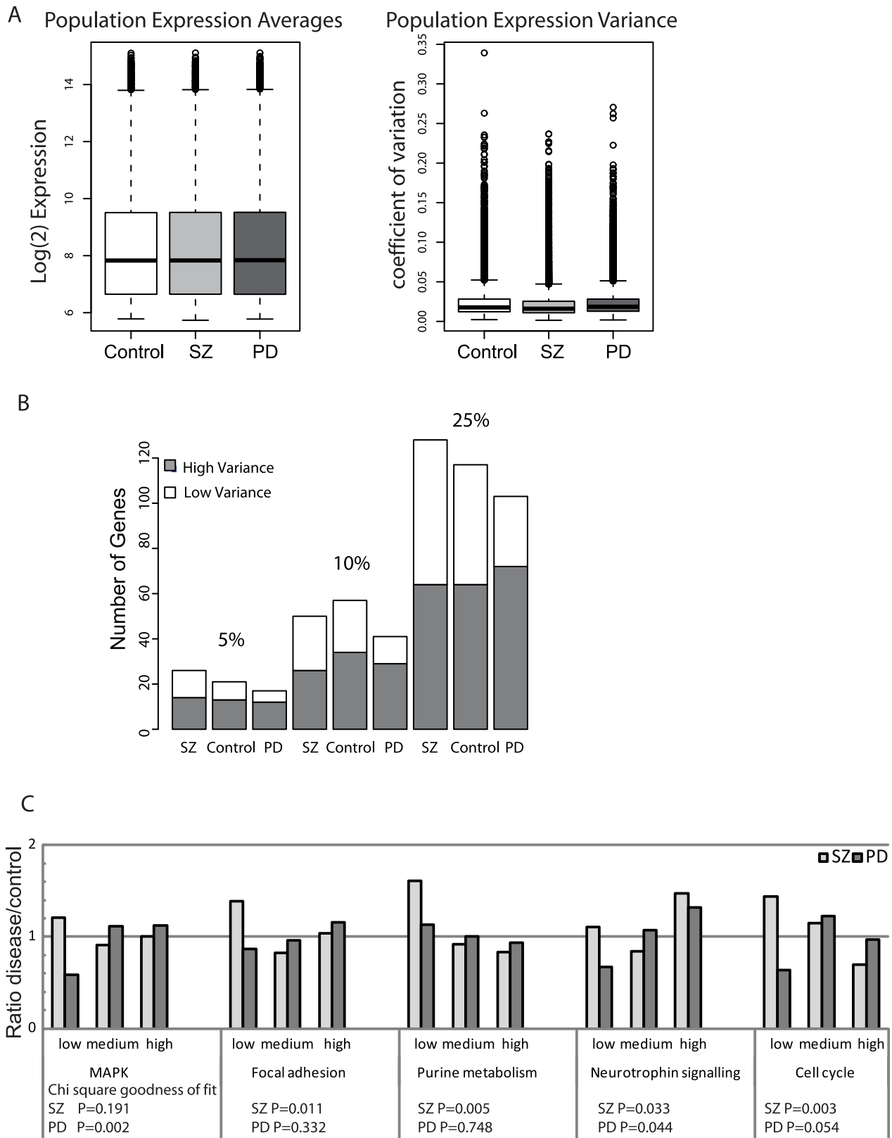
Figure 4. Expression variance discriminates between disease groups. A. Box plots showing whole-genome phenotype-specific mean expression levels and the corresponding CVs for hONS cells derived from the Control, PD, and SZ patient groups. As can be seen, there is no difference in the average \log_2(\text{expression}) measures but noticeable differences in the CVs. Using a two-sample t-test, there is a significant difference between the SZ and Control groups ( p\text{-value} < 2.2 \times 10^{-16} ) and the PD and Control groups ( p\text{-value} < 0.0013 ). B. The observation of increase in high-variance genes for PD and increase in low-variance genes for SZ persists with different percentile cutoffs applied to the variance distribution in the
