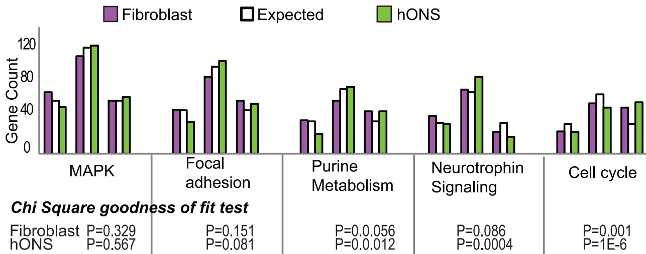
Figure 3. Distribution of variance patterns in the top 5 attract pathways for hONS and fibroblast cells. Chi-square goodness of fit was used to determine if variance profiles differed significantly from the expected 25:50:25% patterns. doi:10.1371/journal.pgen.1002207.g003
