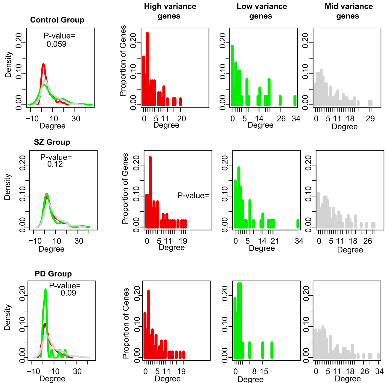
Figure 5. MAPK interaction networks and degree distribution density curves for the highly-constrained (red) and lowly-constrained (green) genes. p-values assess the significance of how different the two degree distributions are. The “Mid Variability” genes, falling between the 25th and 75th percentile of CV values, are shown in gray for comparison. doi:10.1371/journal.pgen.1002207.g005
