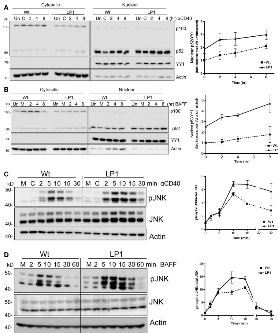
FIGURE 2 | Impact of TRAF3 on CD40 and BAFFR-mediated NF- \kappa B2 and JNK activation. CH12.TRAF3 -/- cells were induced to express Wt or mutant LP1 TRAF3 as in Figure 1. (A,B) Cells were untreated (M) or treated with isotype control Ab (C) or stimulated with 5 \mu g/ml of anti-mouse CD40 mAb (HM40.3) (A) or 200 ng/ml of recombinant BAFF (B) for the indicated times at 37°C. Uninduced cells were also included as control (Un). Cytosolic and nuclear extracts of cell lysates were prepared and immunoblotted for the NF- \kappa B2 precursor protein p100 and its cleavage product p52, with probes for actin and YY1 serving as loading controls for cytoplasmic and nuclear protein levels respectively. YY1 levels were used to normalize nuclear p52 values shown quantitatively in graphs. Representative blots
