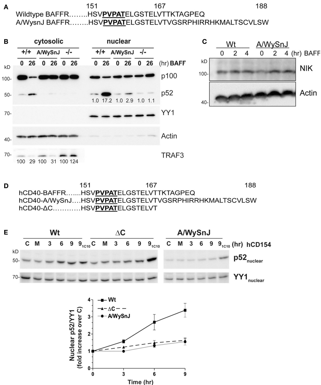
FIGURE 6 | Impaired NF-κB2 activation induced by mutant BAFFRs.
