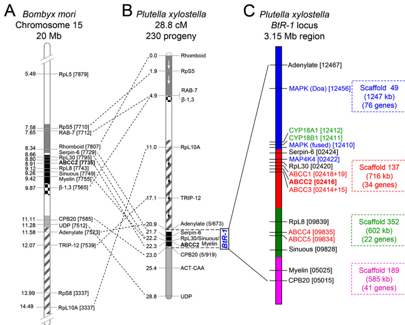
Fig 4. Assembly of the chromosomal region of the BtR-1 resistance locus in P. xylostella . (A) Schematic diagram of partially sequenced chromosome 15 from B. mori . (B) P. xylostella linkage map according to Baxter et al. [10]. Blocks of common genes are shaded and arrows depict inverted orientation in P. xylostella . The dotted lines show multiple chromosomal rearrangements, while maintaining genetic synteny. (C) Detailed genetic makeup of the BtR-1 resistance locus. The four P. xylostella genome scaffolds in BtR-1 are distinguished by color and their information is also listed at the right side. The seven mapped genes were marked out in black (except PxABCC2 in red), all the five PxABCC genes in BtR-1 are denoted in red, three genes in the MAPK signaling pathway are labeled in blue, and two P450 genes are in green. B. mori and P. xylostella gene identifiers refer to the final four or five numbers (note underlining) of the Gene ID corresponding to each genome database (e.g., BGIBMGA007879-TA or Px012467).
