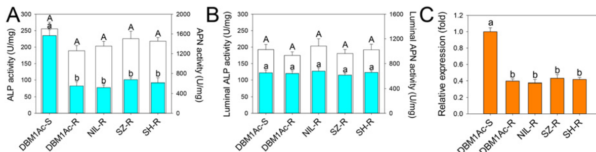
Fig 2. Reduced ALP levels in larval midgut samples from resistant compared to susceptible P. xylostella strains. Specific ALP (2A) and APN (2B) activity was measured in BBMVs (blue bars) or midgut fluids (white bars) from the five P. xylostella strains. Error bar in each column represents standard error of the mean (SEM) from triplicate estimations using three biological replicates. Significant difference for ALP activity was detected between the susceptible strain and all resistant strains ( P < 0.05 ; Holm-Sidak's test; n = 3 ). (C) Relative expression levels of PxmALP as determined by qPCR in midguts of fourth-instar larvae from susceptible and resistant P. xylostella strains. Expression of the ribosomal protein L32 gene was used as the internal reference gene to normalize datasets and calculate relative expression levels, which were calculated assigning a value of 1 to the expression levels in DBM1Ac-S samples. Data shown are the means and corresponding standard errors (SEM) from three biological replicates tested in four technical repeats. Different letters on the bars indicate statistically significant differences in gene expression among strains ( P < 0.05 ; Holm-Sidak's test; n = 3 ).
