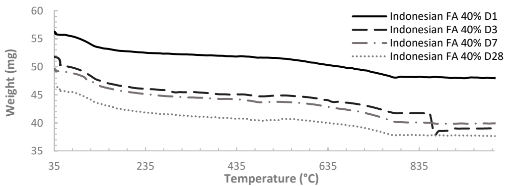
Figure A2. The TG curves for 40% Indonesian fly ash paste at ages of 1, 3, 7 and 28 days.
