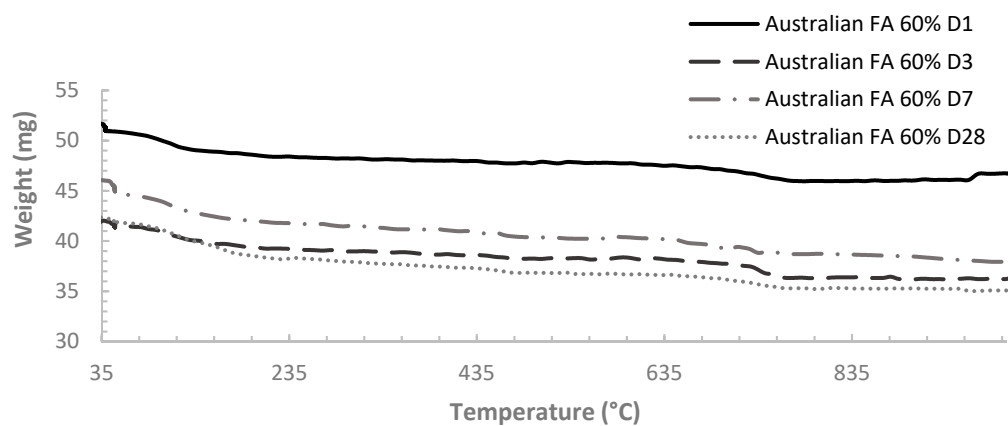
Figure A7. The TG curves for 60% Australian fly ash paste at ages of 1, 3, 7 and 28 days.
