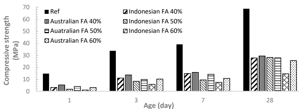
Figure 7. Comparison of compressive strength between Indonesian FA and Australian FA pastes.
