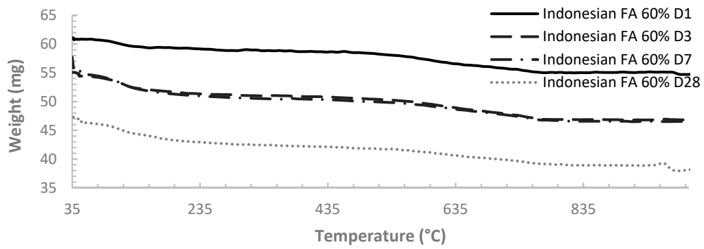
Figure A4. The TG curves for 60% Indonesian fly ash paste at ages of 1, 3, 7 and 28 days.
