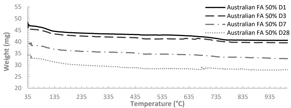
Figure A6. The TG curves for 50% Australian fly ash paste at ages of 1, 3, 7 and 28 days.
