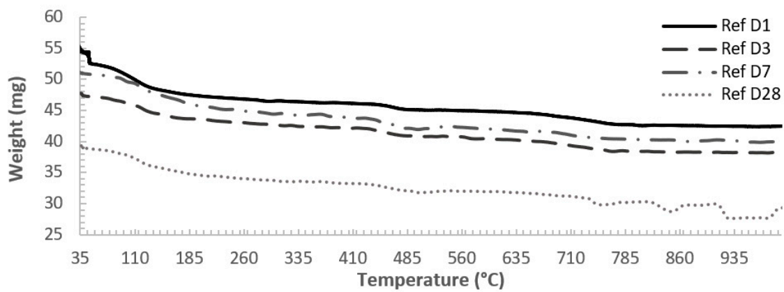
Figure A1. The TG curves for OPC paste at ages of 1, 3, 7 and 28 days.
