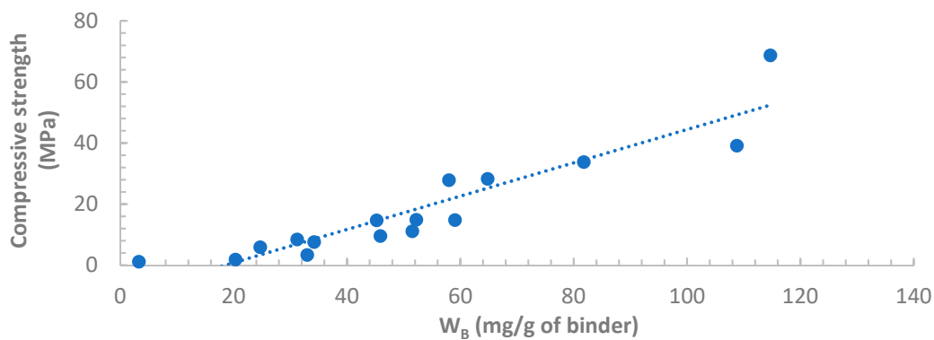
Figure 8. Compressive strength vs. W_B for OPC and Indonesian FA pastes.
