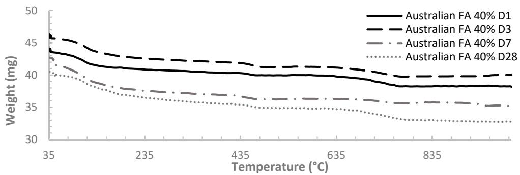
Figure A5. The TG curves for 40% Australian fly ash paste at ages of 1, 3, 7 and 28 days.
