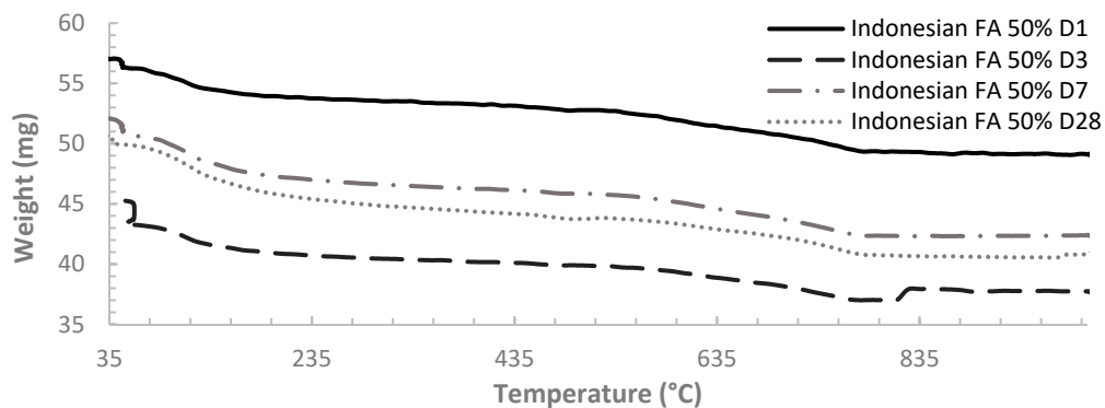
Figure A3. The TG curves for 50% Indonesian fly ash paste at ages of 1, 3, 7 and 28 days.
