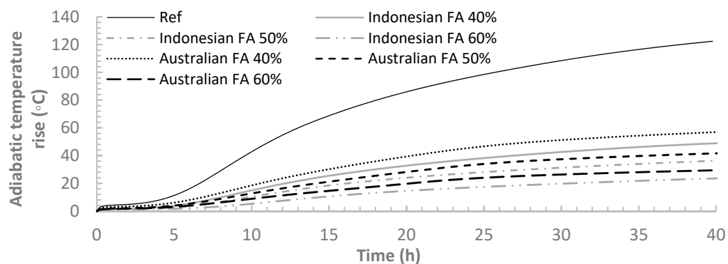
Figure 5. Adiabatic temperature rise for all the paste samples.
