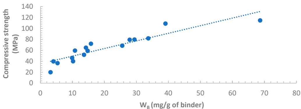
Figure 9. Compressive strength vs. water bound ( W_B ) for OPC and Australian FA pastes.
