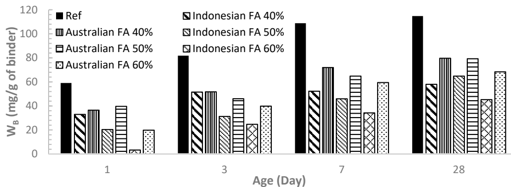
Figure 6. Comparison of W_B between Indonesian FA and Australian FA pastes.
