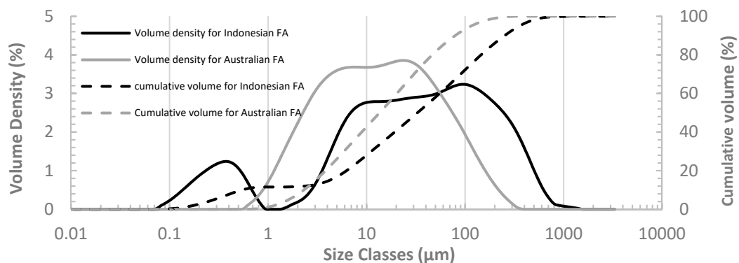
Figure 1. Particle size distribution for both Indonesian FA and Australian FA.
