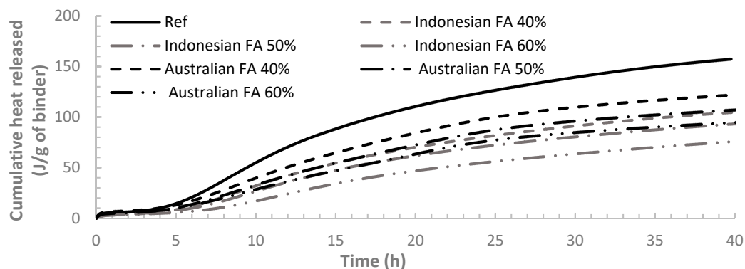
Figure 4. Normalised cumulative heat released for all the cement paste samples.
