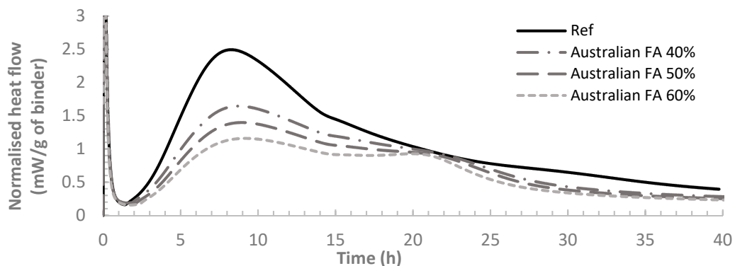
Figure 3. Normalised heat flow for Australian FA and OPC pastes.
