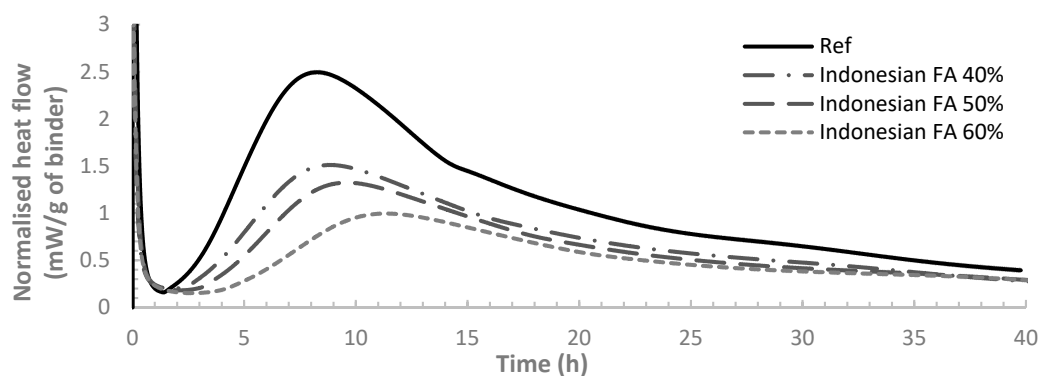
Figure 2. Normalised heat flow for Indonesian FA and OPC pastes.
