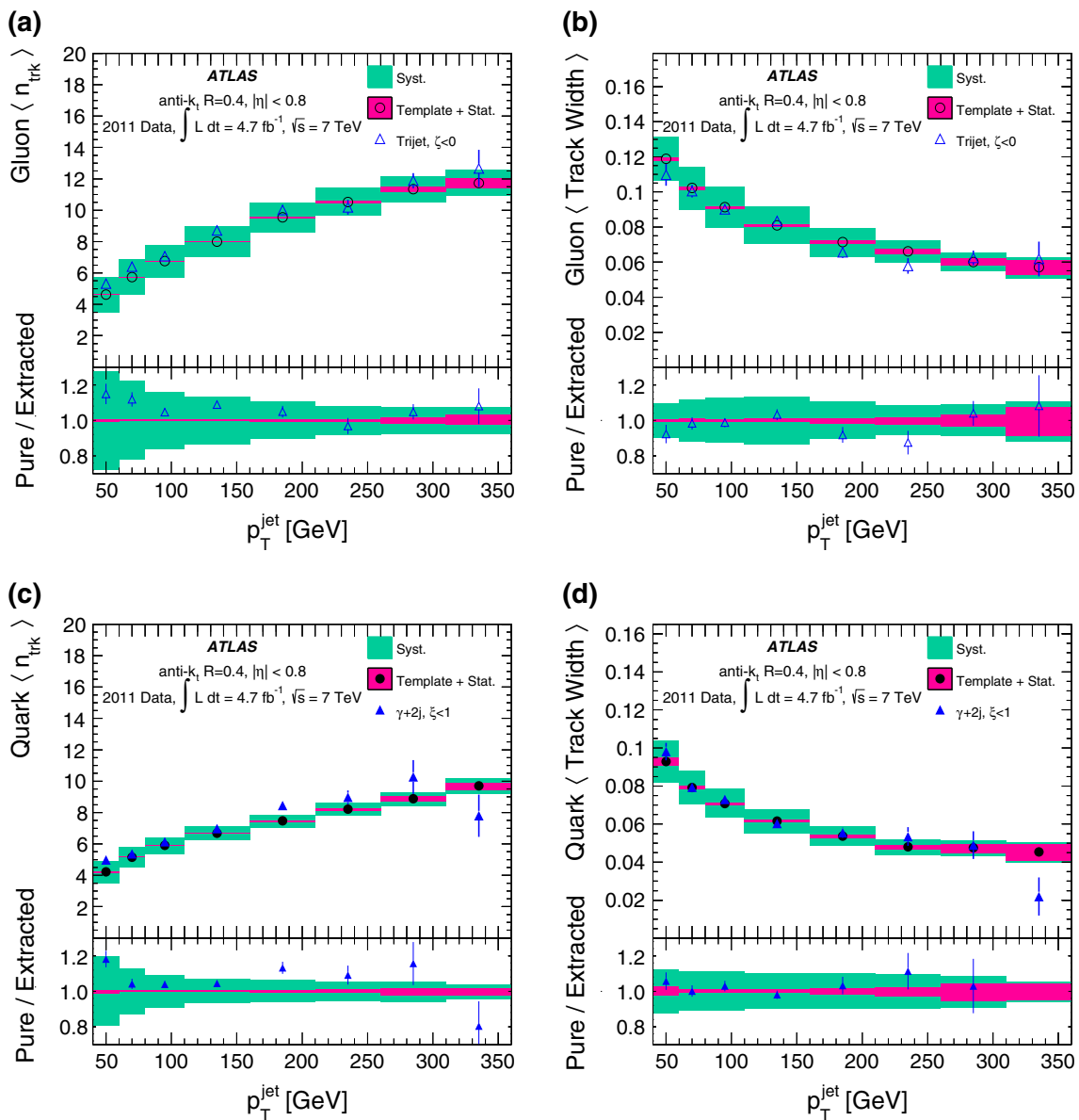
Fig. 3 Top, the jet n_{trk} and b track width as a function of p_T for jets in a gluon-jet-enriched trijet sample (triangles) compared to gluon-jet extracted templates (circles) for |\eta| < 0.8 . Bottom, the jet c n_{trk} and d track width as a function of p_T for jets in a quark-jet-enriched \gamma +jet sample (triangles) compared to quark-jet extracted templates (circles) for jets with |\eta| < 0.8 . Jets are reconstructed with the anti- k_t algorithm
