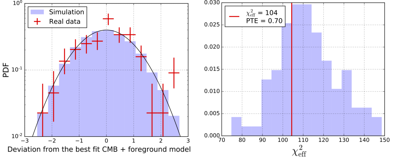
Figure 14. Normalized difference between the measured cross spectra and the best fit CMB+foreground model shown in units of standard deviation (left). Effective \chi_{\text{eff}}^2 of the data fit to the model as defined in Equation 27 compared to simulations (right). The distribution shows the 96 simulations and the vertical line indicates the real data.
