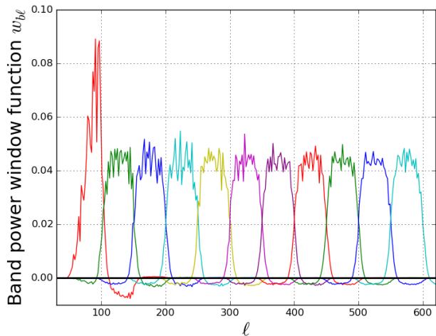
Figure 5. BB band power window functions. The shape of the lowest bandpower is due to the sensitivity degradation at low- \ell due to timestream filtering.
