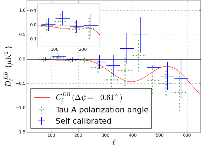
Figure 8. EB power spectrum based on the IRAM Tau A measurement and after polarization angle self-calibration. We find the angle derived from self-calibration to be statistically consistent with PB17. We find our measured EB spectrum to be consistent with zero after an overall polarization angle is subtracted with \chi^2/\nu = 6.56/10 corresponding a 77% PTE. The lowest four bandpowers are shown in the inset.
