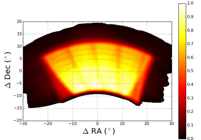
Figure 1. Normalized map depth illustrating the scan pattern centered at (RA, Dec)=( +0^{\text{h}}12^{\text{m}}0^{\text{s}} , -59^{\circ}18' ). The average effective map depth is 32 \mu\text{K}\text{-arcmin} in polarization. The vertical stripes are an artifact of breaks in the low elevation scans to retune the detectors. The horizontal stripes are an artifact of the elevation offsets used in the transit scan. The patch overlaps with the area observed by South Pole experiments.
