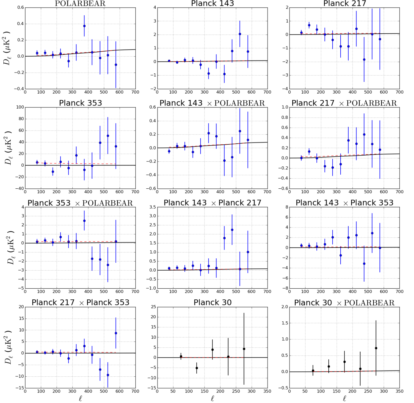
Figure 13. All cross and auto C_{\ell}^{BB} spectra measured in comparison with Planck maps. E-mode spectra are not used in the parameter constraints. Spectra including the Planck 30 GHz maps are indicated with black points and are not used in the fiducial r likelihood. Error bars show the fixed \nu_b approximation. The red dashed curves indicate the best-fit CMB + foreground model. All spectra are shown in CMB temperature units. The black curve indicates the \Lambda\text{CDM} lensing expectation.
