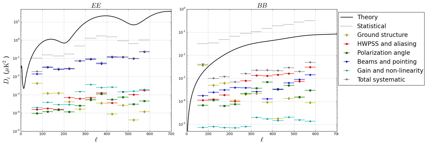
Figure 11. Systematic contributions from all simulated effects grouped thematically for EE and BB , left and right. The ground structure curve indicates the sum of contamination from the detector gain and linear drift models of ground contamination. The HWPSS and aliasing curve includes 0f and 2f signal aliasing as well as the HWP imperfections. The polarization angle curve shows the sum of individual and overall polarization angle uncertainties after self calibration. The beams and pointing curve includes pointing model uncertainty and effects related to detector crosstalk. The gain and non-linearity curve includes relative gain uncertainty and detector gain and time constant drift acting on the CMB signal. The dominant effect in EE is the misestimation of the effective polarization beam due to detector crosstalk while the dominant systematic in BB is the uncertainty in the ground structure subtraction. It should be noted that this is a conservative estimate driven by significant model uncertainties. Future experiments may be able to suppress this effect significantly through careful study and control of ground pickup. The total systematic error is formed assuming all systematics add linearly in power.
