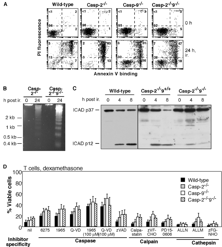
Figure 4. Dying caspase-2 -/- 9 -/- cells display hallmarks of apoptosis and are protected by caspase inhibitors but not calpain/cathepsin inhibitors. (A–C) Ly5.1 - CD4 + 8 + thymocytes sorted from reconstituted mice were cultured following 5 Gy \gamma irradiation (ir.). (A) Staining with FITC-conjugated Annexin V plus PI reveals phosphatidylserine exposure before loss of membrane integrity irrespective of genotype. (B) DNA “laddering” indicative of inter-nucleosomal fragmentation demonstrated by gel electrophoresis of genomic DNA. (C) Western blots showing processing of ICAD in dying caspase-2 -/- 9 -/- cells. (D) The death of caspase-2 -/- 9 -/- cells is antagonized by inhibitors of caspases but not of calpains or cathepsins. Ly5.1 - Thy1 + mature T lymphocytes from the lymph nodes of reconstituted mice were cultured for 24 h in the presence of 100 nM dexamethasone plus the caspase inhibitors zVAD-fmk, IDN-6275 (6275), IDN-1965 (1965), or Q-VD-OPH (Q-VD), the calpain inhibitors z-VF-CHO or PD-150606, a cell permeable peptide of the calpain inhibitor calpastatin, the dual calpain/cathepsin inhibitors ALLM and ALLN or the cathepsin inhibitor z-FG-NHO-Bz-pOME (zFG-NHO) (each at 50 \mu M). Cell death was quantified by PI staining and FACS analysis. Results represent mean \pm SD of at least three independent experiments for each genotype. Vehicle: 0.4% DMSO.
