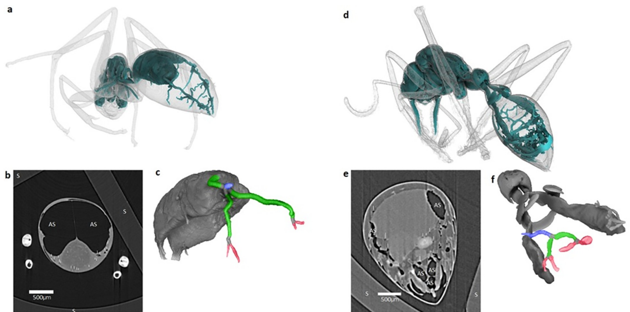
Fig 2. Results of the reconstruction of x-ray tomography of a Camponotus suffusus minor (a-c), and Myrmecia fulvipes (d-f). (a, d) Volume render of the body and internal airspaces (cyan). (b, e) Horizontal planar slice of the abdomen with air sacs (AS) and tracheal branches (white vertical line) indicated, the mounting syringe (S) is visible around the edges of the images. Additional examples of the raw slices for other ant genera can be found in S3 Fig. (c, f) Volume render of the internal airspace showing the air sac and associated trachea branches, coloured by their respective level as in Fig 1 (blue, green, red for tracheal levels 1, 2, 3, respectively, as in Fig 1). Note perspective distortions arising from presenting a three-dimensional volume in two dimensions. The radii of each branch shown for C. suffusus (c) were measured as 29.15 \mu\text{m} (blue), 13.87, 10.11, 5.59 \mu\text{m} (green), and 6.35, 8.02, 5.40, 5.24 \mu\text{m} (red). The radii of each branch shown for M. fulvipes (f) were measured as 32.83 \mu\text{m} (blue), 17.67, 14.44 \mu\text{m} (green), and 11.78, 8.13, 6.19, 6.61 \mu\text{m} (red).
