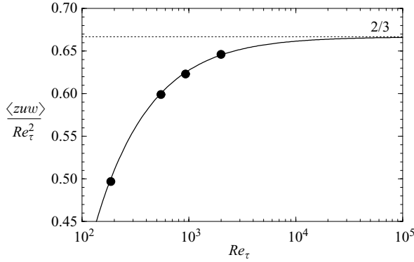
FIGURE 3. Formulation for \langle z\overline{uw} \rangle (using (3.13)) as a function of Re_\tau . The solid circles correspond to the DNS data as in figure 2.
