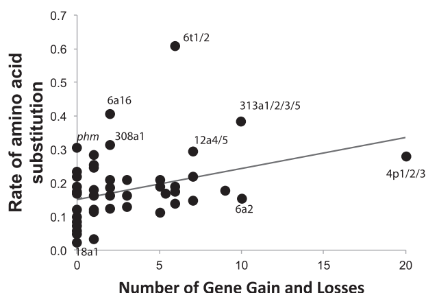
FIG. 8. —The relationship between gene gain/loss and rate of amino acid substitution. The x axis represents the number of gene gain and losses in the AncD clades. The y axis is the rate of amino acid substitution accounting for changes in evolutionary time due to gene gain and losses.
