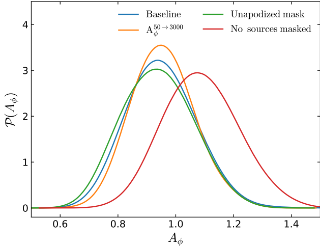
Figure 13. Constraints on A_\phi given various changes to the analysis as compared to the baseline result.
