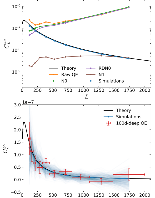
Figure 5. Bandpowers and noise terms from the quadratic estimate (QE) pipeline. The top panel shows the normalized but noise-biased QE, along with the N_L^{(0)} , N_L^{(0, \text{RD})} , and N_L^{(1)} noise terms, computed via Monte Carlo. The blue curve is the average of cross spectra between simulations and true \phi maps, and is used to compute the Monte Carlo correction, f_{\text{PS}} . The bottom panel shows the noise-bias-subtracted QE and error bars (from simulations), as well as the same blue simulation line as in the top plot, now with a cloud of blue lines denoting each individual simulation.
