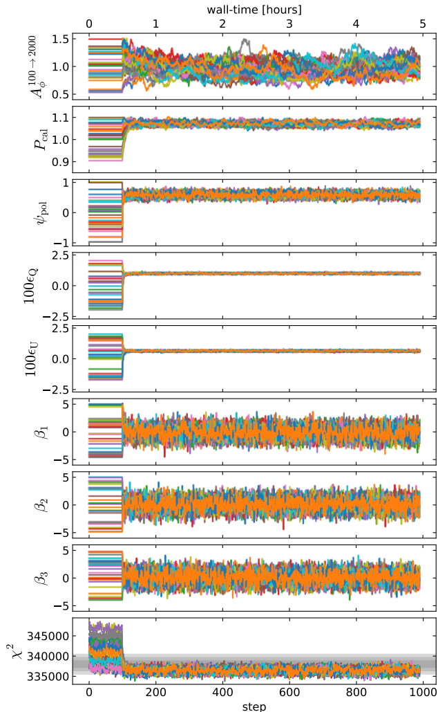
Figure 6. The top 8 plots show the trace of the sampled cosmological and systematic parameters, \theta , at each step in the Monte Carlo chain. The very bottom plot shows the trace of the \chi^2 of the current model point, along with a gray shaded band indicating the expectation based on the number of degrees of freedom. Note that 202,800 other parameters are jointly sampled in this chain (not pictured), corresponding to every pixel or Fourier mode in the CMB polarization and \phi maps. To aid convergence, the \theta are not updated for the first 100 steps in the chain. These 32 independent chains ran across 4 Tesla V100 GPUs in roughly 5 hours.
