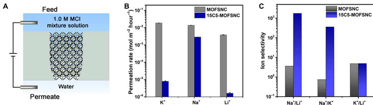
Fig. 3. Ion permeation rate and selectivity of MOFSNC and 15C5-MOFSNC. (A) Schematics of the experimental setup for ion permeation under multicomponent conditions where a transmembrane voltage is applied to drive ion transport from the feed (base side) to the permeate side (tip side). (B and C) Permeation rate and selectivity of the MOFSNC and 15C5-MOFSNC in multicomponent solutions with an applied voltage bias of 1.0 V.
