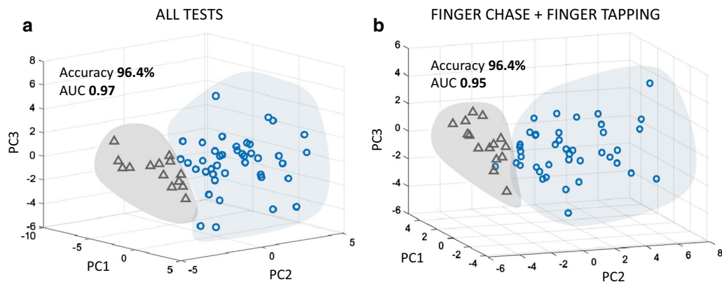
Fig. 4 Group classification in PCA. a All features. b FCT and FTT features
