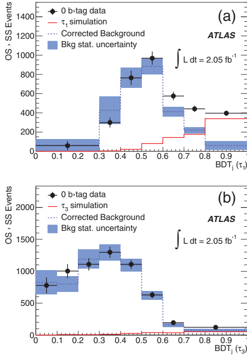
Figure 1: BDT_j (OS-SS) distributions of \ell + \tau ( e and \mu combined) events in the 0 b -tag data (black points): (a) \tau_1 (b) \tau_3 . The expected contributions from \tau and e (sum of Z \rightarrow \tau^+ \tau^- , single top and \tilde{t}\bar{t} \rightarrow \ell + \tau + X ) are shown as a solid red line. The derived background templates after applying MC corrections are shown as dashed histogram with shaded/blue statistical uncertainty bands. The shapes of these background templates are used for the fits to the \geq 1 b -tag distributions.
