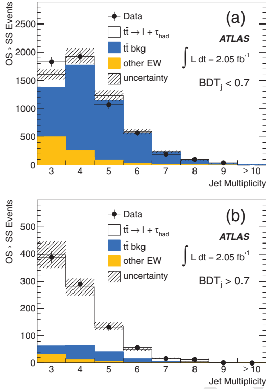
Figure 3: OS-SS number of jets distributions for events with at least one b -tag. The \mu + \tau and e + \tau channels have been summed together. The solid circles indicate data and the histograms indicate the expected signal and backgrounds. The normalisation of the expected signal and the backgrounds are based on the fit result. The uncertainty includes statistical and systematic contributions. The fraction of each background is estimated from MC. (a) is for \text{BDT}_j < 0.7 , (b) for \text{BDT}_j > 0.7 .
