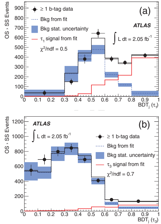
Figure 2: BDT_j (OS-SS) distributions of \ell + \tau in the \geq 1 b -tag sample; (a) \tau_1 , (b) \tau_3 . The normalisation of each template is derived from a fit to the data. The fitted contributions are shown as the light/red (signal), dashed/blue (background derived from 0 b -tag data after applying MC corrections) and dark/black (total) lines. Shaded/blue bands are the statistical uncertainty of the background template.
