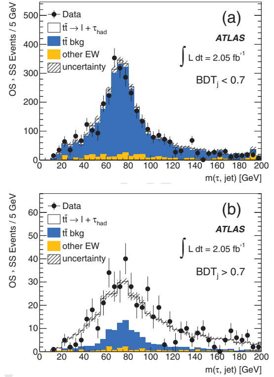
Figure 4: OS-SS invariant mass of jet and \tau candidate for events with at least one b -tag. The jet is the highest p_T untagged jet in events with more than one b -tag and the second highest p_T untagged jet in events with one b -tag. The \mu + \tau and e + \tau channels have been summed together. The solid circles indicate data and the histograms indicate the expected signal and backgrounds. The normalisation of the expected signal and the backgrounds are based on the fit result. The uncertainty includes statistical and systematic contributions. The fraction of each background is estimated from MC. (a) is for \text{BDT}_j < 0.7 , (b) for \text{BDT}_j > 0.7 .
