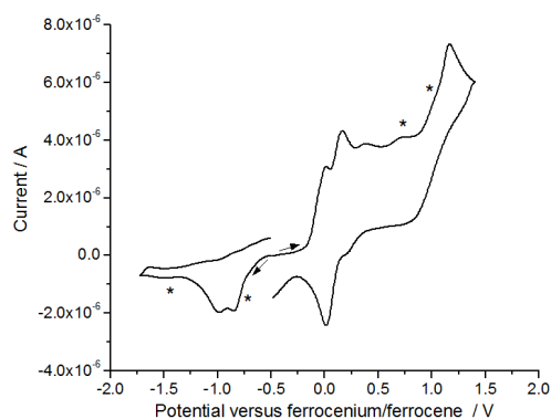
Figure 3. Cyclic voltammograms of 5b in acetonitrile (1.0 mM with 0.1 M Bu 4 NPF 6 ) measured with a 1.0 mm diameter glassy carbon working electrode
