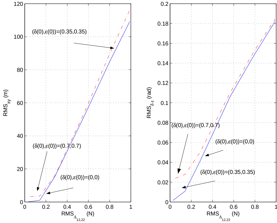
Figure 10. The impact of exogenous noises upon the performance
