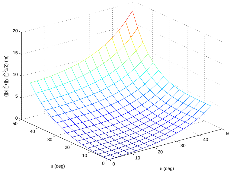
Figure 9. Overshoot \sqrt{\|x\|_\infty^2 + \|y\|_\infty^2} against the angles (\delta, \epsilon)
