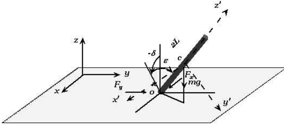
Figure 1. The spherical inverted pendulum
