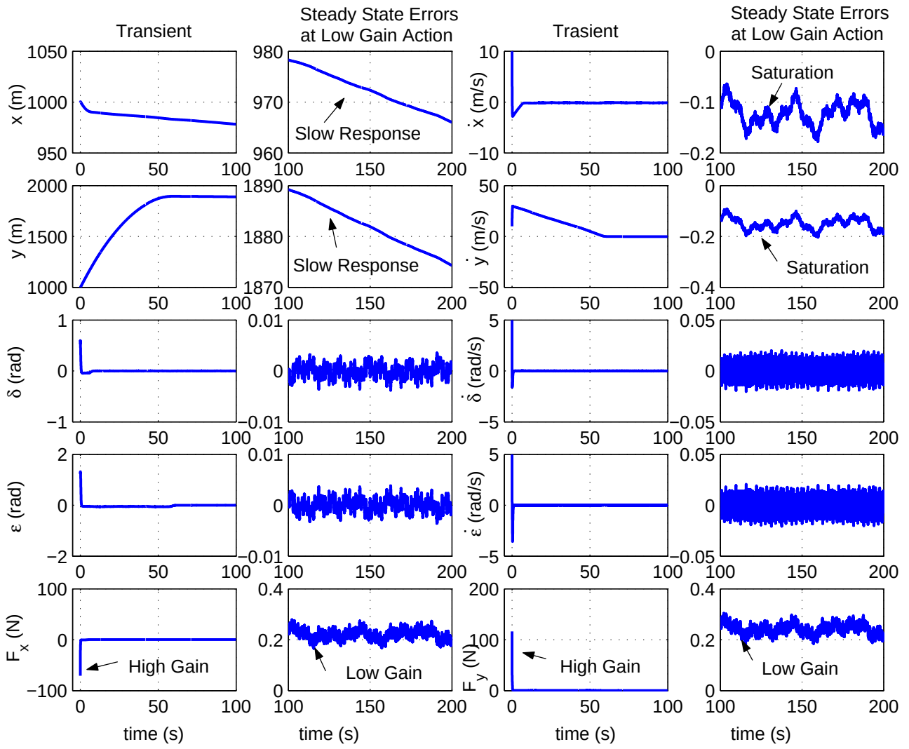
Figure 5. Simulation Results for Case 3
