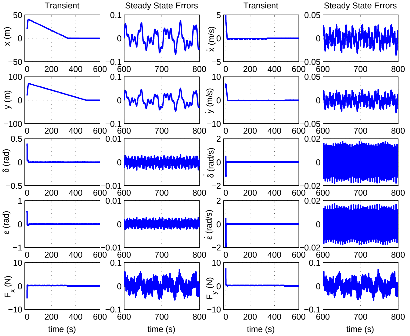
Figure 4. Simulation Results for Case 2
