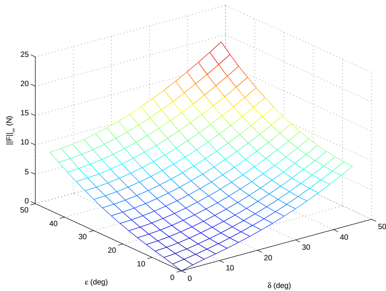
Figure 6. \|F\|_\infty against the angles (\delta, \epsilon)
