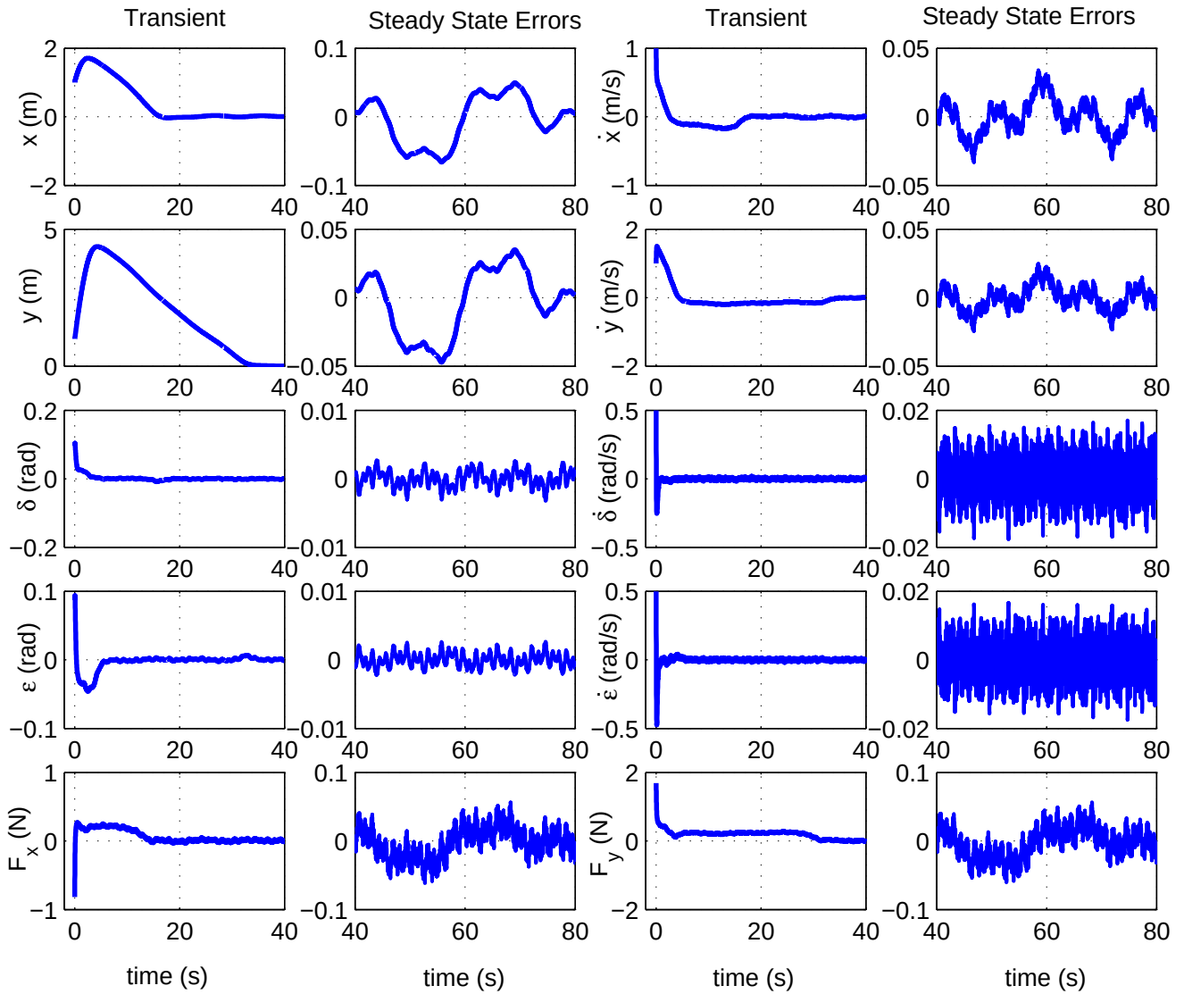
Figure 3. Simulation Results for Case 1
