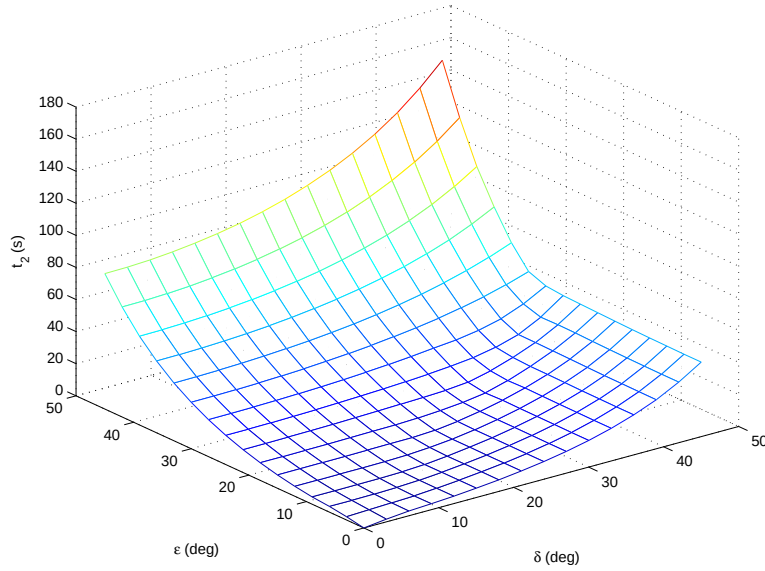
Figure 8. Time t_2 to the origin against the angles (\delta, \epsilon)
