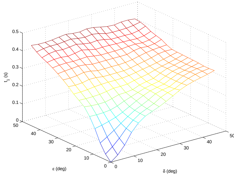
Figure 7. Time t_1 to the upright position against the angles (\delta, \epsilon)
