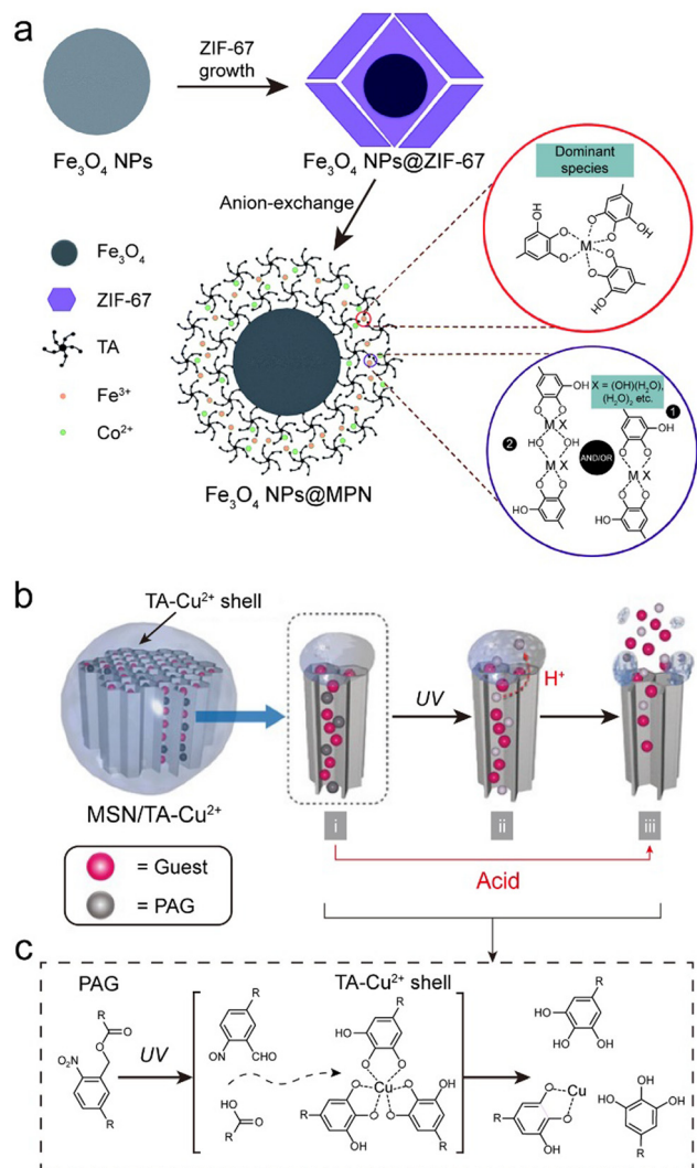
Fig. 17 (a) Schematic illustration of the synthesis of Fe 3 O 4 @MPN composites. Adapted with permission from ref. 154. Copyright 2019, Royal Society of Chemistry. (b) and (c) Gating activity and adhesion of TA and TA-Cu 2+ complexes on the surface of MSN. (b) Schematic and (c) mechanism of decomposition of MPNs (Cu 2+ -TA) by photoacid generators (PAGs) in MPN-MSN composites. (b) and (c) Adapted with permission from ref. 155. Copyright 2017, Wiley-VCH.
