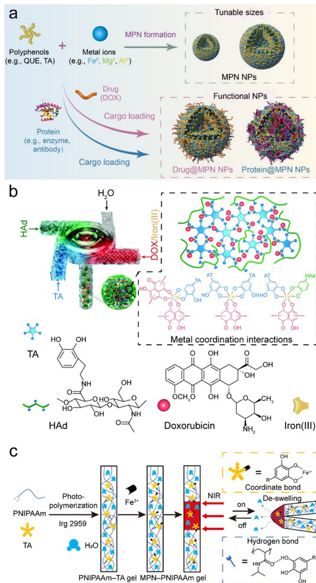
Fig. 10 (a) Complexation method for forming MPN composites. NPs, nanoparticles. Reproduced with permission from ref. 69. Copyright 2023, Xu et al. , published by Wiley-VCH GmbH. (b) Coordination-driven rapid complexation of MPN-dopamine-modified hyaluronic acid (HAD)-DOX nanoparticle composites using a turbulent mixing device. Reproduced with permission from ref. 78. Copyright 2019, Royal Society of Chemistry. (c) Synthesis and NIR-triggered actuation (reversible bending-unbending) of MPN-PNIPAAm composite hydrogels. Adapted with permission from ref. 42. Copyright 2021, American Chemical Society.
