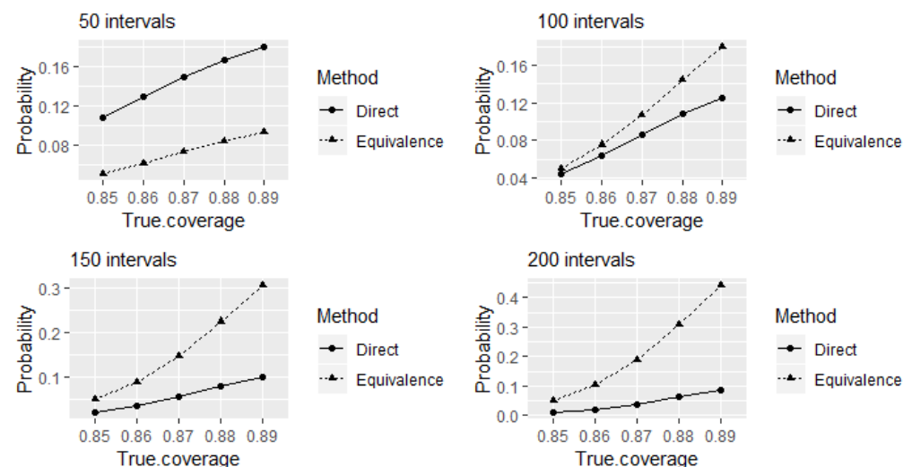
Figure 2. The probabilities of the direct and equivalence tests to identify the experts as 90% well-calibrated when true levels of coverage of elicited intervals that are less than 90%.
