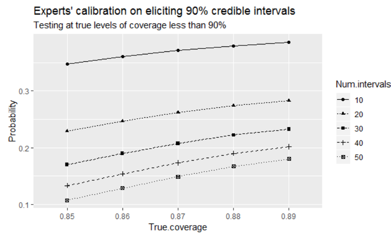
Figure 3. The probabilities of the direct test to identify the experts as 90% well-calibrated when true levels of coverage of elicited intervals that are less than 90% for small number of elicited intervals.
