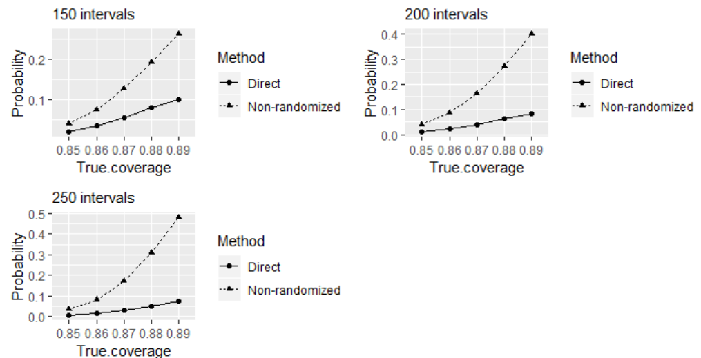
Figure 6. The probabilities of the direct and non-randomized equivalence tests to identify the experts as 90% well-calibrated when true levels of coverage of elicited intervals that are less than 90%.
