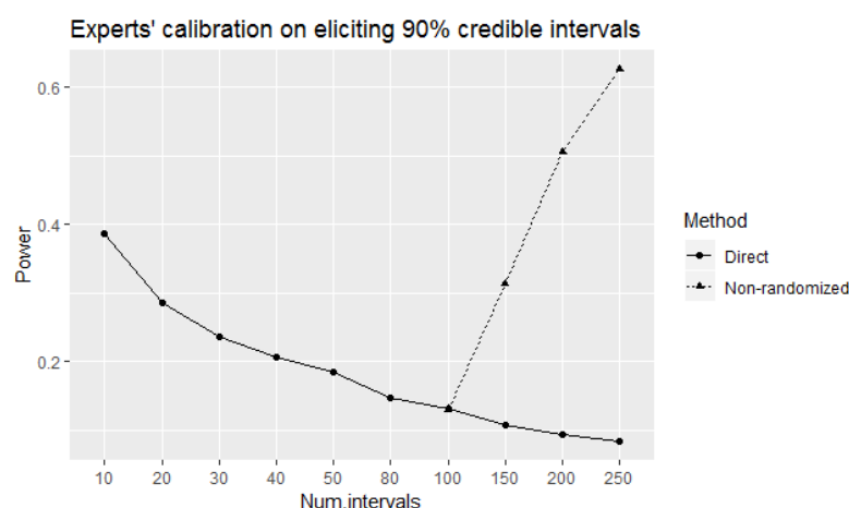
Figure 5. The power of the direct and non-randomized equivalence tests to correctly identify 90% well-calibrated experts at 90% true level of coverage of elicited intervals.
