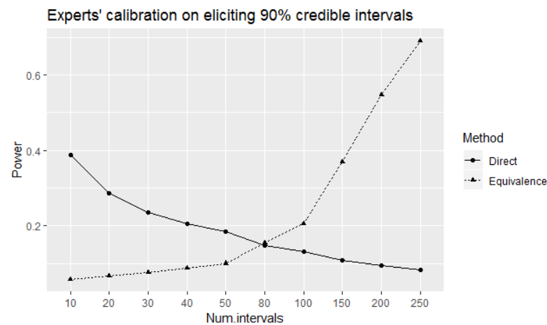
Figure 1. The power of the direct and equivalence tests to correctly identify 90% well-calibrated experts at 90% true level of coverage of elicited intervals.
