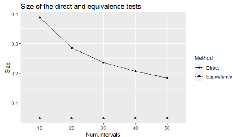
Figure 4. Size of the direct and equivalence tests in testing experts' calibration on eliciting 90% credible intervals for small number of elicited intervals.
