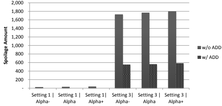
Figure 9: Amount of spoilage taking (or not) into consideration age dependent demand for instances of Settings 1 and 3 when varying \alpha_k .
