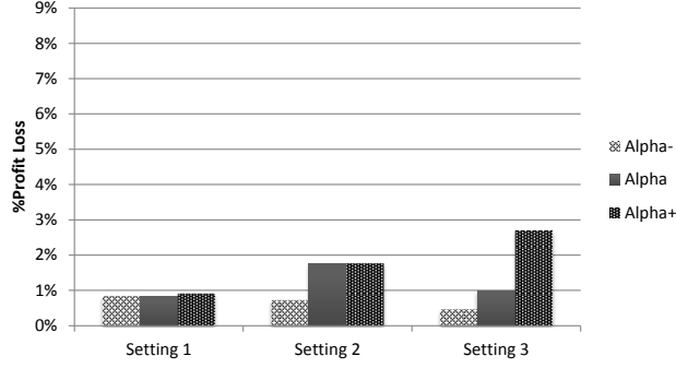
Figure 11: Profit loss due to neglecting consumer purchasing behaviour of picking up the fresher products available for all Settings varying \alpha_k .
