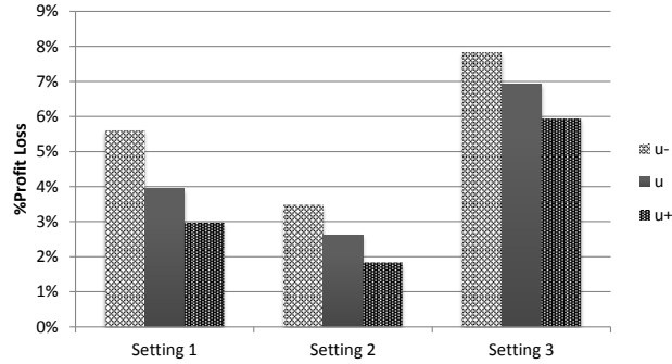
Figure 8: Profit loss due to neglecting age dependent demand for all Settings varying u_k .
