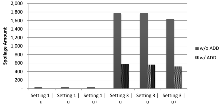
Figure 10: Amount of spoilage taking (or not) into consideration age dependent demand for instances of Settings 1 and 3 when varying u_k .
