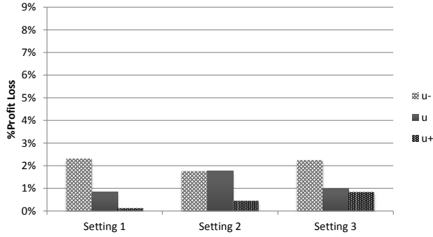
Figure 12: Profit loss due to neglecting consumer purchasing behaviour of picking up the fresher products available for all Settings varying u_k .
