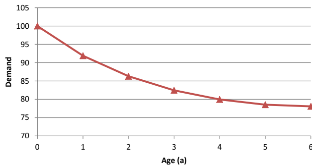
Figure 4: Example of the demand curve for beef over its shelf-life of 7 days, starting at 100 units. According to Tsiros & Heilman (2005) beef has a high PQR, \alpha = 0.52 , \hat{p} = 2.68 and p^0 = 2.52 ; and according to Andreyeva et al. (2010) it has \epsilon = -0.75 .
