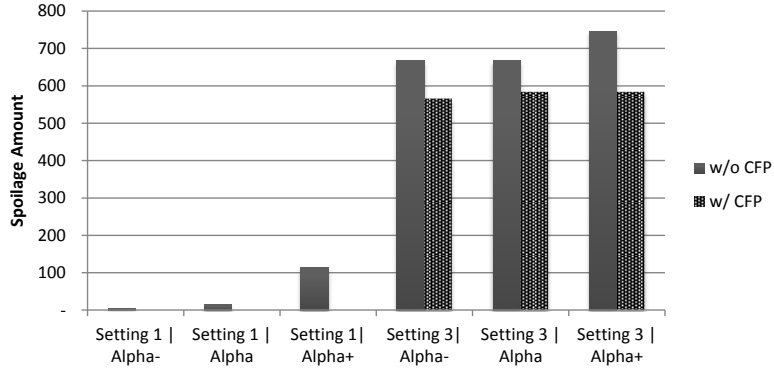
Figure 13: Amount of spoilage taking (or not) into consideration customer's eagerness for fresher products for instances of Settings 1 and 3 when varying \alpha_k .
