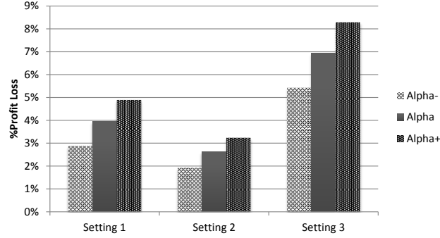
Figure 7: Profit loss due to neglecting age dependent demand for all Settings varying \alpha_k .
