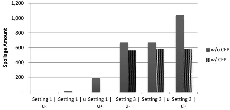
Figure 14: Amount of spoilage taking (or not) into consideration customer's eagerness for fresher products for instances of Settings 1 and 3 when varying u_k .
