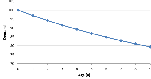
Figure 3: Example of the demand curve for lettuce over its shelf-life of 10 days, starting at 100 units. According to Tsiros & Heilman (2005) lettuce has a medium PQR, \alpha = 0.62 , \hat{p} = 2.49 and p^0 = 2.86 ; and according to Andreyeva et al. (2010) it has \epsilon = -0.58 .
