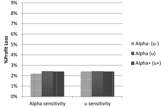
Figure 15: Profit loss due to assuming a medium PQR for all products of Setting 3 varying \alpha_k and u_k .
