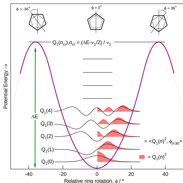
Figure 3. Schematic representation of the potential energy surface along the Q_1 normal coordinate. Harmonic oscillator wavefunctions, their square and \langle Q_1(n)^2, \phi_{0-36} \rangle are shown for the lowest levels of Q_1 .
