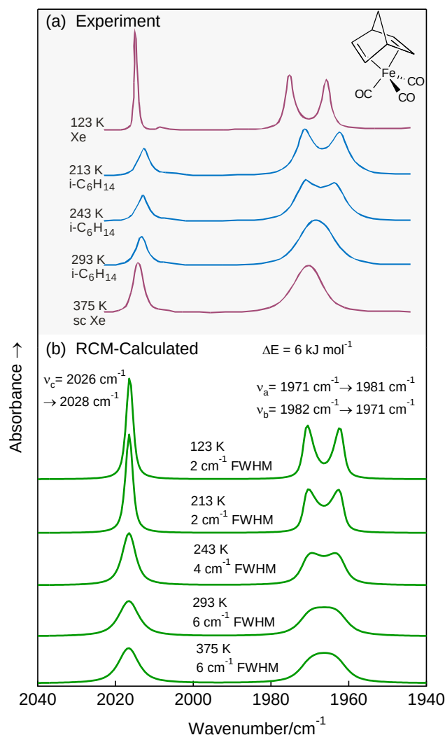
Figure 6. (a) Experimental and (b) RCM-Calculated IR spectra of (\text{NBD})\text{Fe}(\text{CO})_3 . The calculated spectra use the DFT-calculated spectra for the ground and transition states from ref. [23] and the experimental spectra are redrawn from the spectra presented by Turner et al. [17b] and Giodarno and Lear [18b] and were obtained either as matrix-isolated samples in Xe or as solutions in 2-methylpentane ( i\text{-C}_6\text{H}_{14} ) or supercritical Xe.
