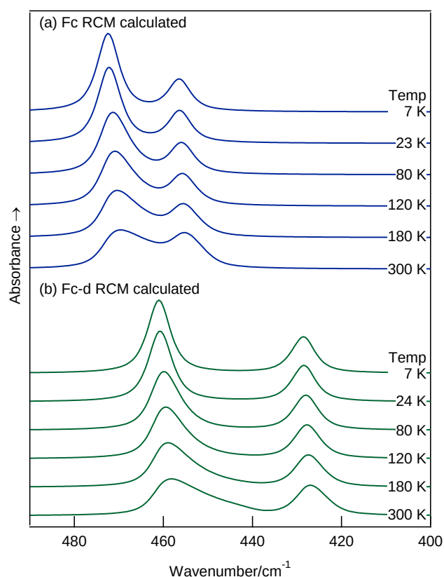
Figure 5. Temperature dependence of the RCM-calculated IR spectra of (a) Fc and (b) Fc-d using the gas-phase DFT calculated wavenumbers and intensities of Q_7 and Q_{8,9} of the D_{5h} and D_{5d} forms of Fc. Spectra of Fc-d were calculated by applying the \nu_H/\nu_D calculated for the respective normal modes. Values of \Delta E and \nu_1 were set to 6 kJ mol -1 and 25 cm -1 , respectively.
