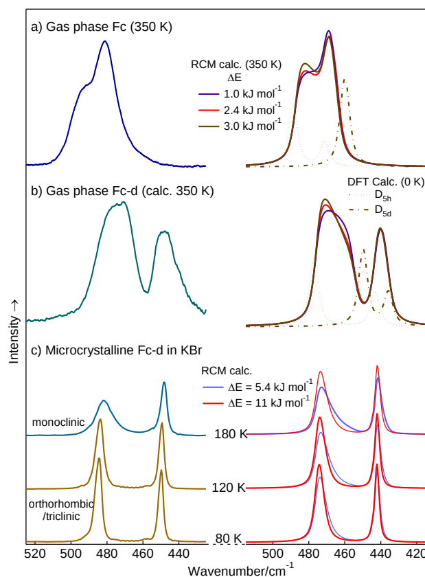
Figure 4. Experimental and calculated IR spectra of gas phase spectra of (a) Fc and (b) Fc-d and (c) microcrystalline Fc-d in KBr. RCM-calculated spectra were obtained using the DFT calculated values of v_1 and v_7 , I(Q_7) , v_{8,9} and I(Q_{8,9}) of D_{5h} and v_7 and v_{8,9} of D_{5d} gas-phase Fc/Fc-d (shown). For gas-phase spectra a FWHM of 6 \text{ cm}^{-1} was used for all component bands. For the microcrystalline sample the FWHM of v_7 and v_{8,9} were set to 2.5 and 5 \text{ cm}^{-1} , respectively. Other parameters (temperature, \Delta E ) are as indicated.
