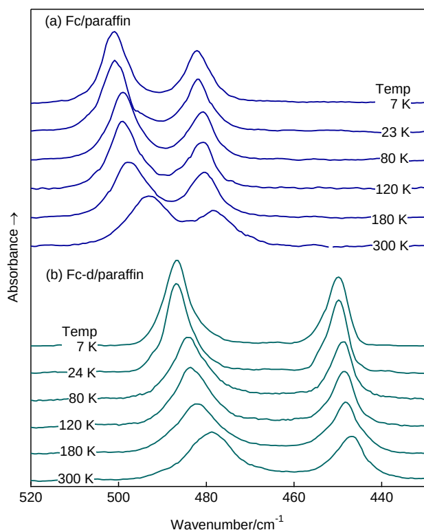
Figure 2. Temperature-dependent IR spectra of (a) Fc and (b) Fc-d as dilute frozen solutions in paraffin. The lower intensity, lower-wavenumber band is assigned to Q_7 and the higher-wavenumber band assigned to Q_{8,9} .
