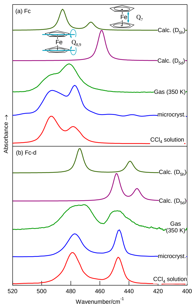
Figure 1. IR spectra of (a) Fc and (b) Fc-d. The DFT-calculated spectra are for the \text{CCl}_4 -solvated molecule and are drawn with a symmetric band profile with 6 \text{cm}^{-1} FWHM. Experimental spectra were obtained at ca. 300 K (condensed phases) or 350 K (gas phase). Microcrystalline samples were prepared as KBr discs. The Q_7 and Q_{8,9} modes are shown for D_{5h} Fc..
