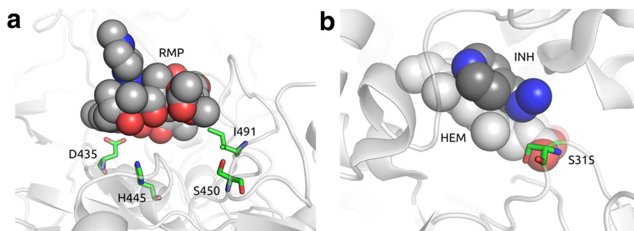
Fig. 4 Mutations in binding site regions. a depicts the spatial distribution of mutated residues in the rpoB -RMP complex while (b) shows the residue Ser315 in katG -INH complex (residues depicted with carbons in green). The distance between the residues and the ligands (depicted with carbons in dark grey) vary from 2.1 to 5.7 Å. RMP rifampicin, INH isoniazid
