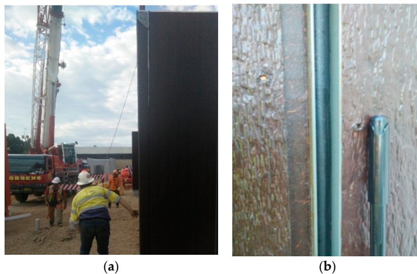
Figure 17. Lifting and placement of panels: (a) Complete prefabricated wall panels are lifted and place into position whilst compressing the rubber gasket; (b) Due diligence in measurement of gap width and assessment of shape and embedment depth.
