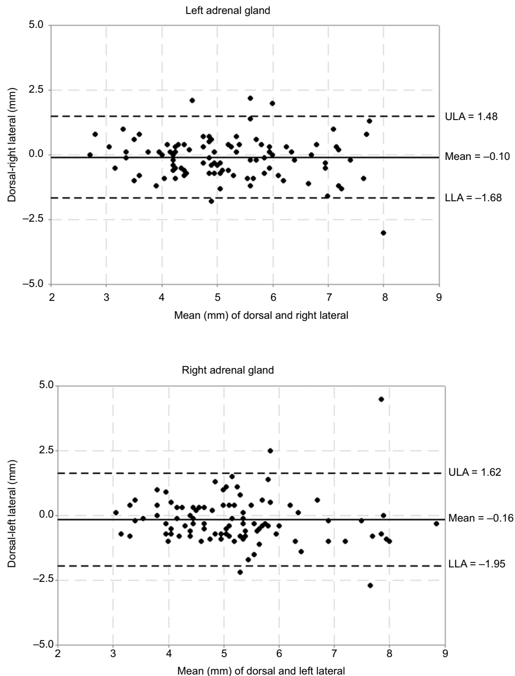
Figure 2 Graphical display of the Bland–Altman analysis of the caudal pole thickness measurement acquired from the longitudinal image plane of the left and right adrenal gland.
