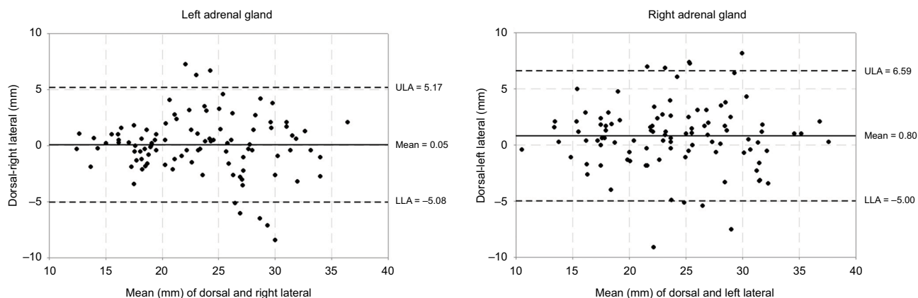
Figure S3 Bland-Altman Plot for the length of the adrenal gland.
