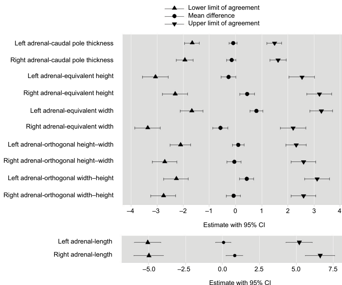
Figure 3 Adrenal gland measurements.
